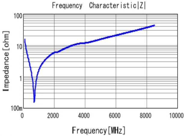
■ GRM2165C2A101JA01 |Z| DCOV, 25degC
