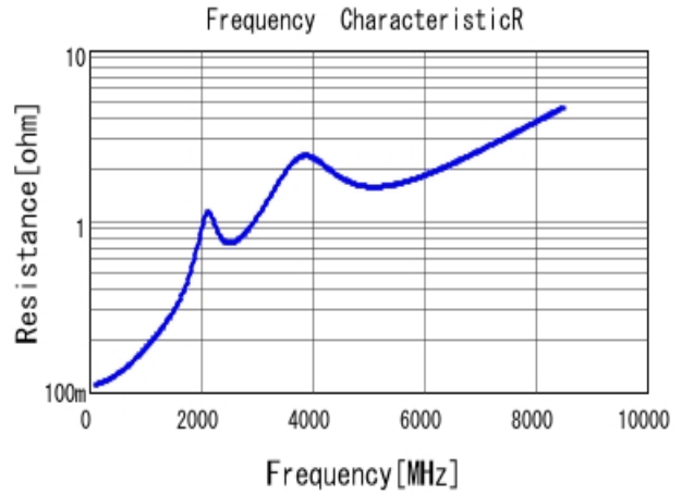
■ GRM2165C2A101JA01 R DCOV, 25degC
