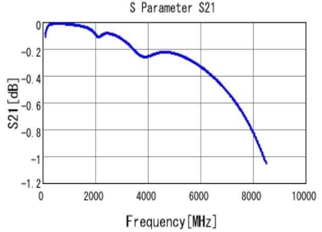
■ GRM2165C2A101JA01 S21 DCOV, 25degC
