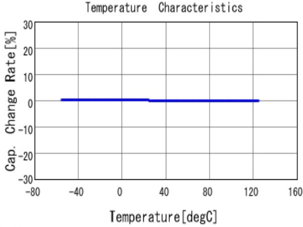
■ GRM2165C2A101JA01 C-Temp. capchange, DCOV, AC1Vrms
