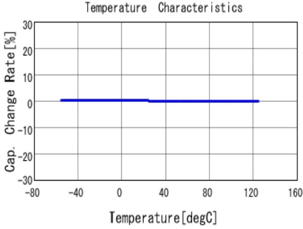
■ GRM2165C1H472JA01 C-Temp. capchange, DCOV, AC1Vrms
