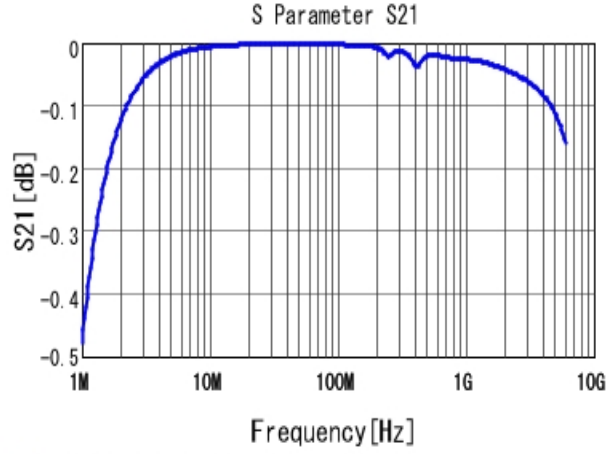
■ GRM2165C1H472JA01 S21 DCOV, 25degC
