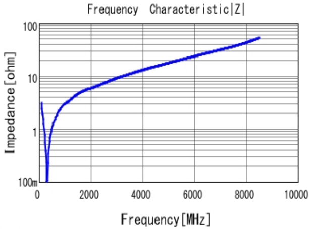
■ GRM2165C1H471JA01 |Z| DCOV, 25degC
