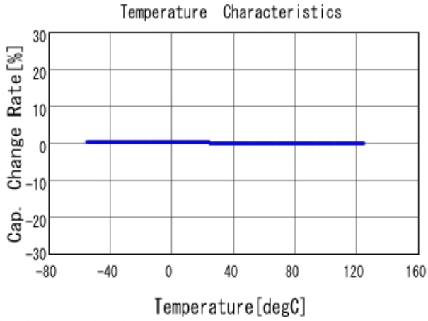
■ GRM2165C1H392JA01 C-Temp. capchange, DCOV, AC1Vrms
