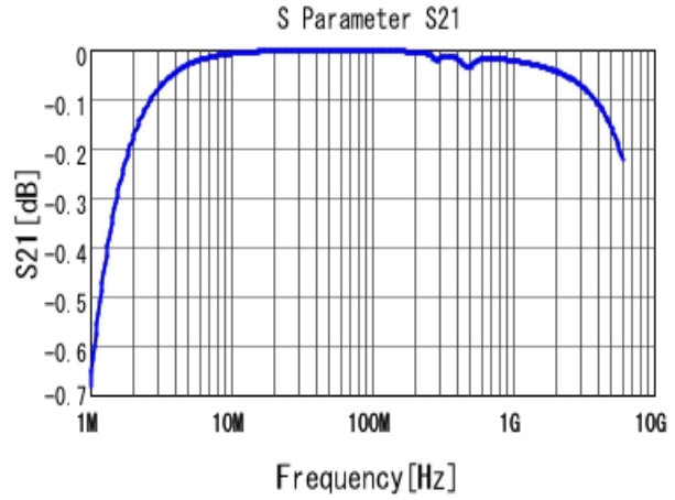
■ GRM2165C1H392JA01 S21 DCOV, 25degC
