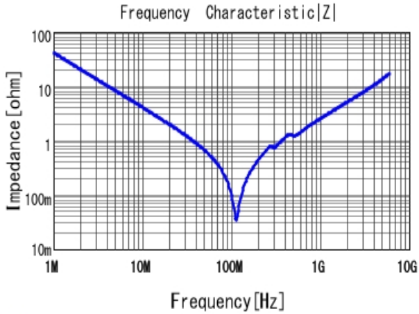
■ GRM2165C1H392JA01 |Z| DCOV, 25degC
