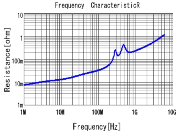
■ GRM2165C1H392JA01 R DCOV, 25degC
