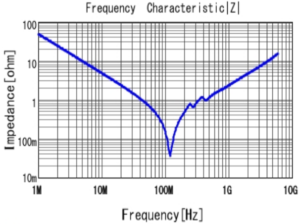
■ GRM2165C1H332JA01 |Z| DCOV, 25degC
