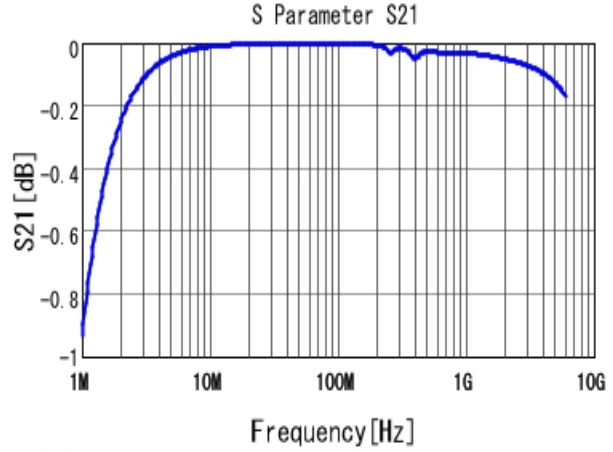
■ GRM2165C1H332JA01 S21 DCOV, 25degC
