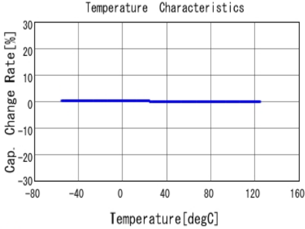
■ GRM2165C1H332JA01 C-Temp. capchange, DCOV, AC1Vrms
