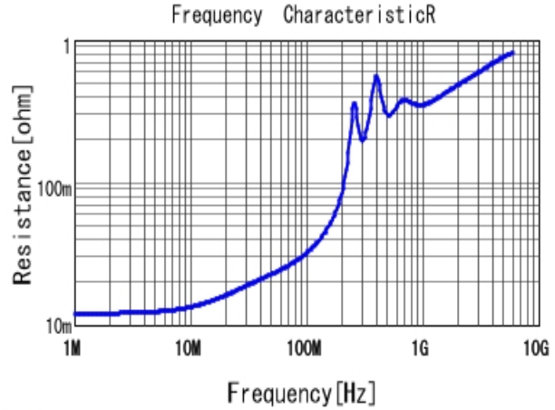
■ GRM2165C1H332JA01 R DCOV, 25degC
