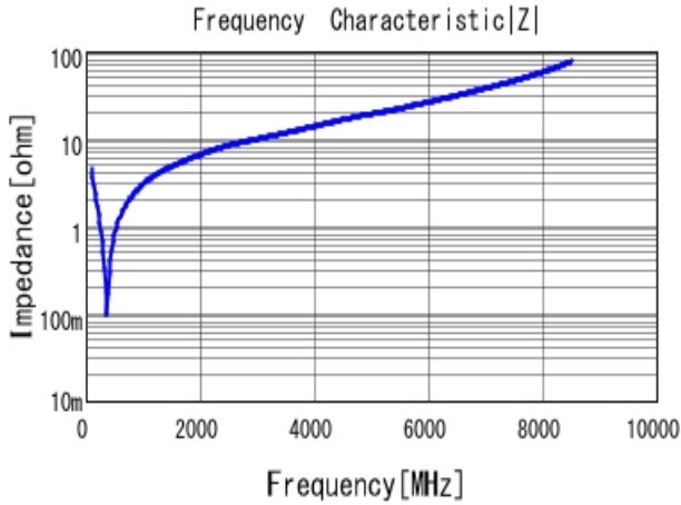
■ GRM2165C1H331JA01 |Z| DCOV, 25degC
