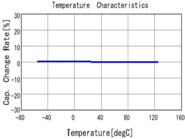
■ GRM2165C1H331JA01 C-Temp. capchange, DCOV, AC1Vrms
