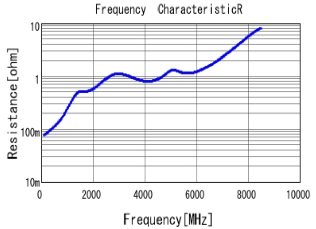
■ GRM2165C1H331JA01 R DCOV, 25degC
