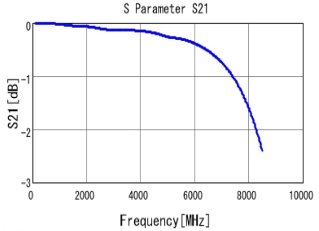
■ GRM2165C1H331JA01 S21 DCOV, 25degC
