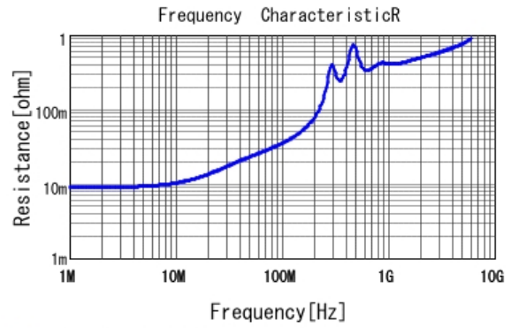
■ GRM2165C1H272JA01 R DCOV, 25degC
