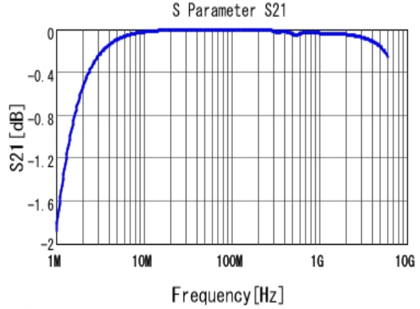
■ GRM2165C1H222JA01 S21 DCOV, 25degC
