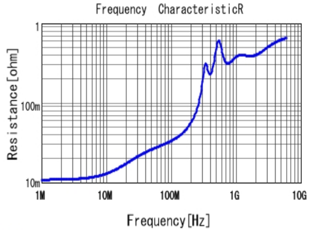
■ GRM2165C1H222JA01 R DCOV, 25degC
