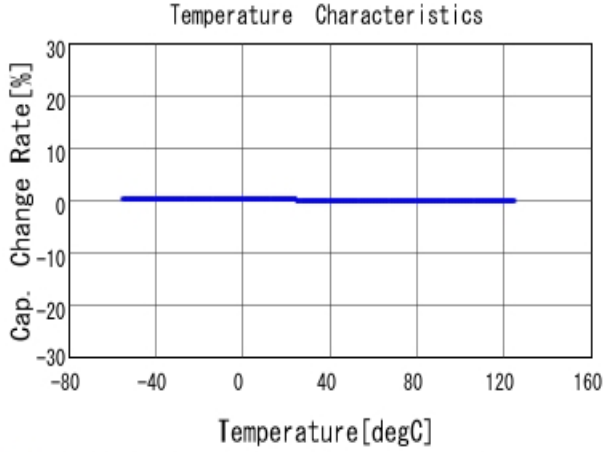
■ GRM2165C1H222JA01 C-Temp. capchange, DCOV, AC1Vrms
