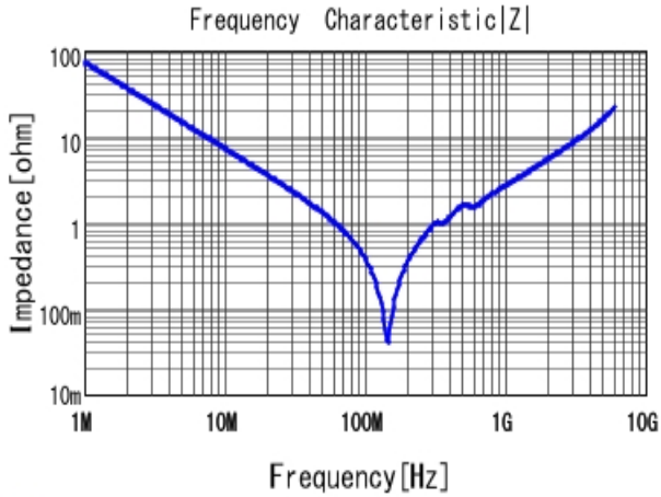
■ GRM2165C1H222JA01 |Z| DCOV, 25degC
