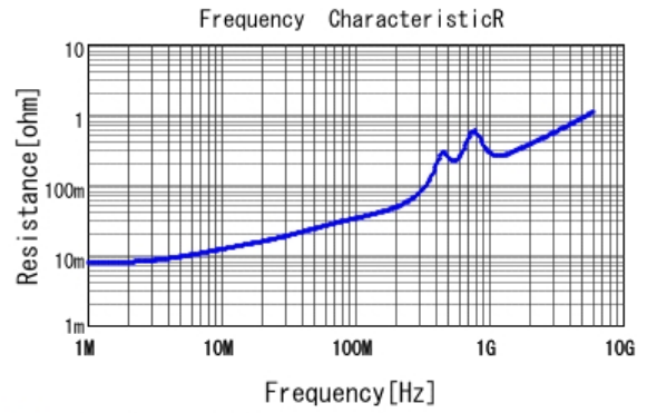
■ GRM2165C1H182JA01 R DCOV, 25degC
