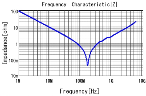
■ GRM2165C1H182JA01 |Z| DCOV, 25degC
