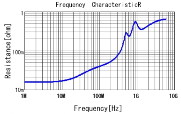
■ GRM2165C1H152JA01 R DCOV, 25degC
