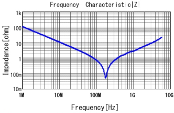
■ GRM2165C1H152JA01 |Z| DCOV, 25degC
