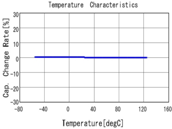
■ GRM2165C1H122JA01 C-Temp. capchange, DCOV, AC1Vrms
