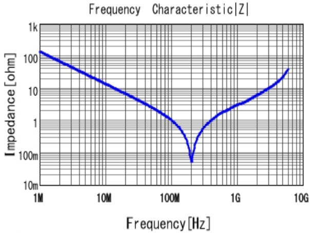
■ GRM2165C1H122JA01 |Z| DCOV, 25degC
