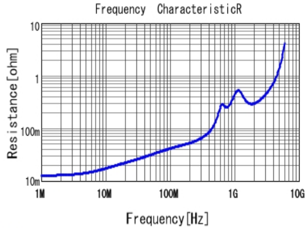
■ GRM2165C1H122JA01 R DCOV, 25degC
