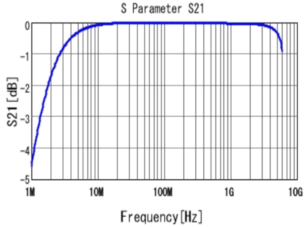
■ GRM2165C1H122JA01 S21 DCOV, 25degC
