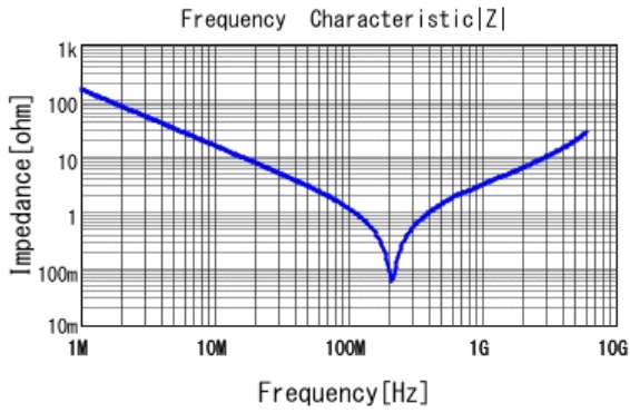
■ GRM2165C1H102JA01 |Z| DCOV, 25degC
