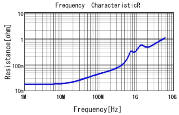
■ GRM2165C1H102JA01 R DCOV, 25degC
