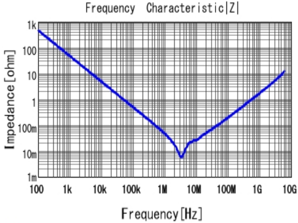
■ GRM188Z71C475KE21 |Z| DCOV, 25degC
