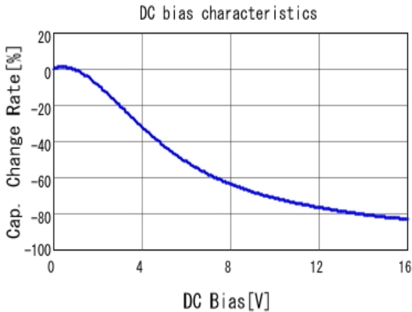
■ GRM188Z71C475KE21 C-DC bias capchange, 25.0degC, AC1V
