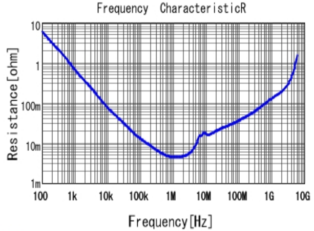
■ GRM188Z71C475KE21 R DCOV, 25degC
