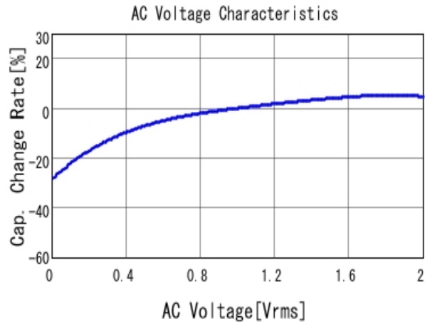
■ GRM188Z71C475KE21 C-AC Voltage capchange, DCOV, 25.0d
