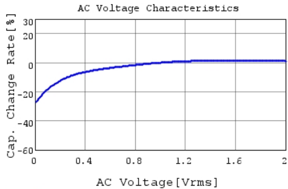
GRM188Z71A106KA73 C-AC Voltage capchange, Dc
