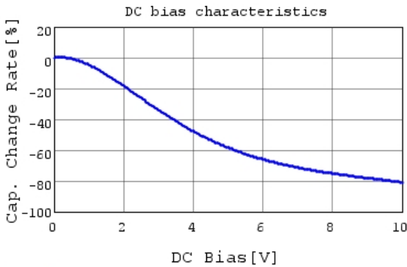
GRM188Z71A106KA73 C-DC bias capchange, 25.0c
