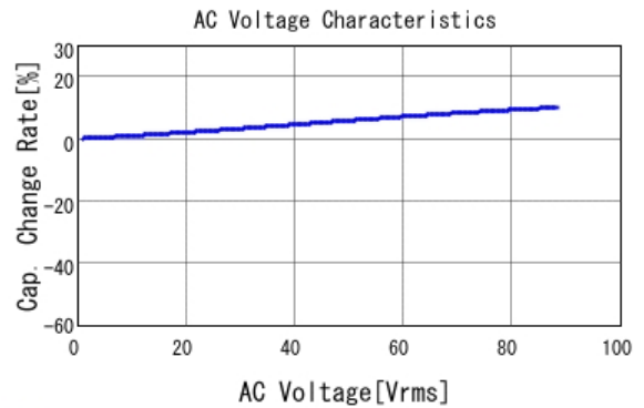
■ GRM188R72E221KW07 C-AC Voltage capchange, DCOV, 25.0d
