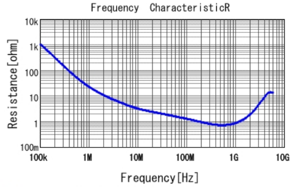
■ GRM188R72E221KW07 R DCOV, 25degC
