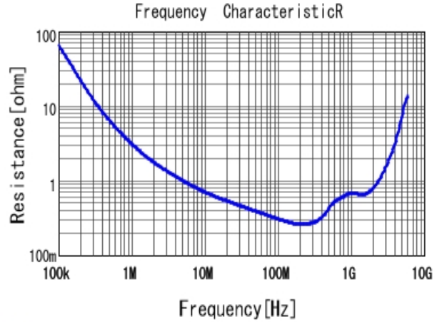
■ GRM188R72E102KW07 R DCOV, 25degC
