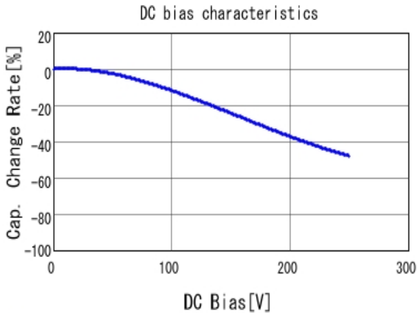
■ GRM188R72E102KW07 C-DC bias capchange, 25.0degC, AC1V
