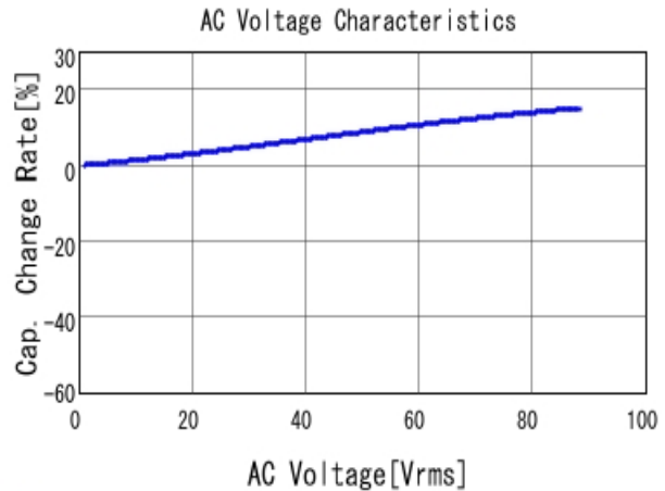
■ GRM188R72E102KW07 C-AC Voltage capchange, DCOV, 25.0d
