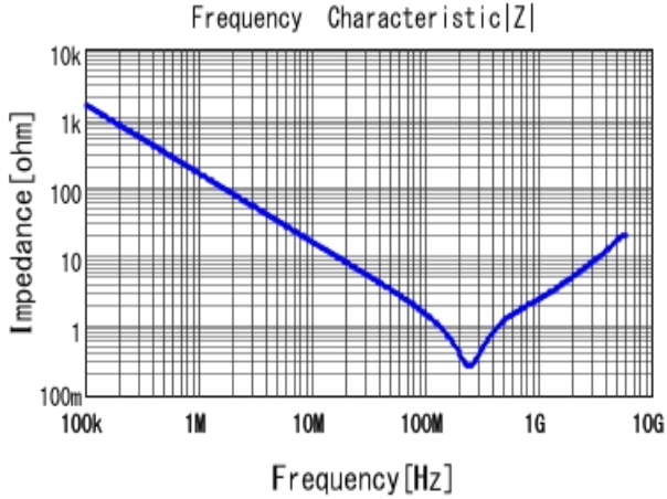
■ GRM188R72E102KW07 |Z| DCOV, 25degC
