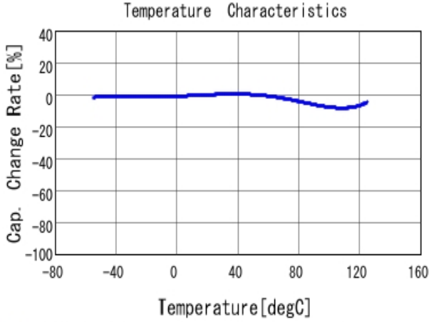
■ GRM188R72E102KW07 C-Temp. capchange, DCOV, AC1Vrms
