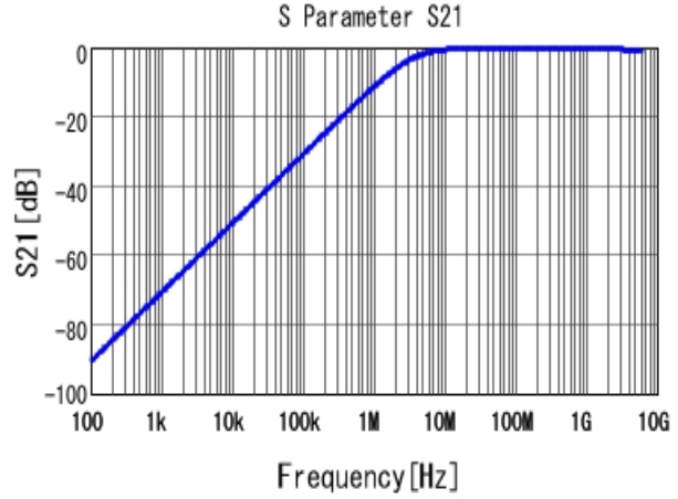
■ GRM188R72A471KA01 S21 DCOV, 25degC
