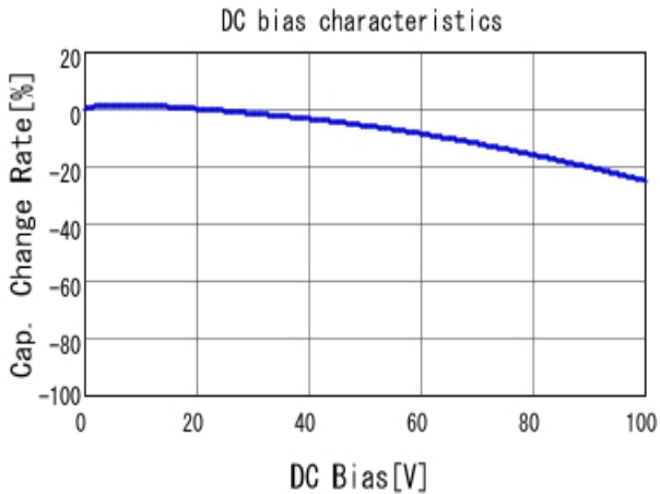
■ GRM188R72A471KA01 C-DC bias capchange, 25.0degC, AC1.
