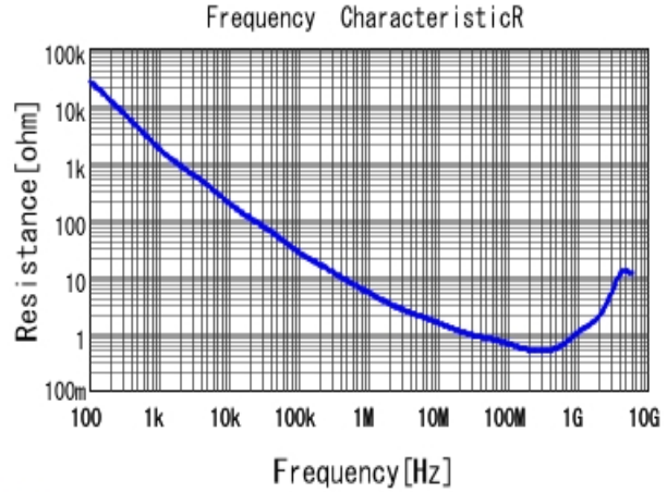
■ GRM188R72A471KA01 R DCOV, 25degC
