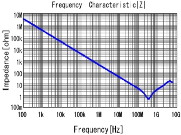
■ GRM188R72A471KA01 |Z| DCOV, 25degC
