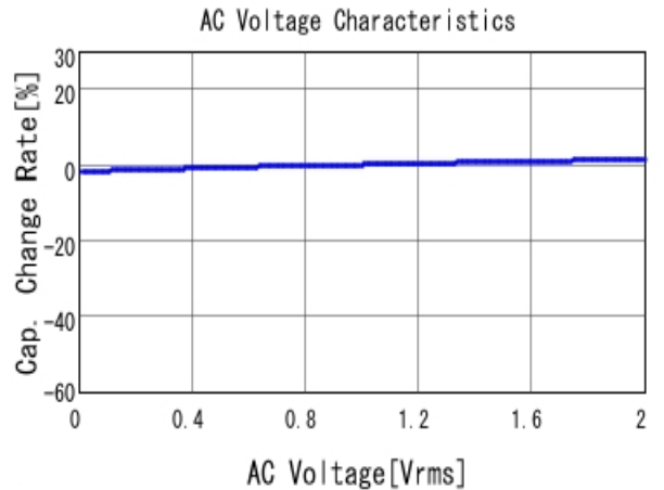
■ GRM188R72A471KA01 C-AC Voltage capchange, DCOV, 25.0d
