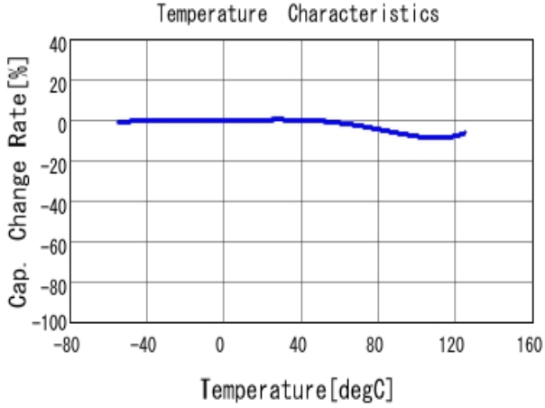
■ GRM188R72A471KA01 C-Temp. capchange, DCO. 0V, AC1. 0Vrm
