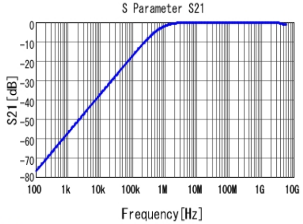
■ GRM188R72A222KA01 S21 DCOV, 25degC
