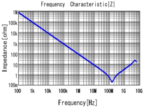
■ GRM188R72A222KA01 |Z| DCOV, 25degC
