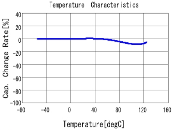
■ GRM188R72A222KA01 C-Temp. capchange, DCO. 0V, AC1.0Vrm
