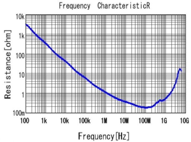
■ GRM188R72A222KA01 R DCOV, 25degC
