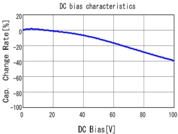
■ GRM188R72A222KA01 C-DC bias capchange, 25.0degC, AC1.
