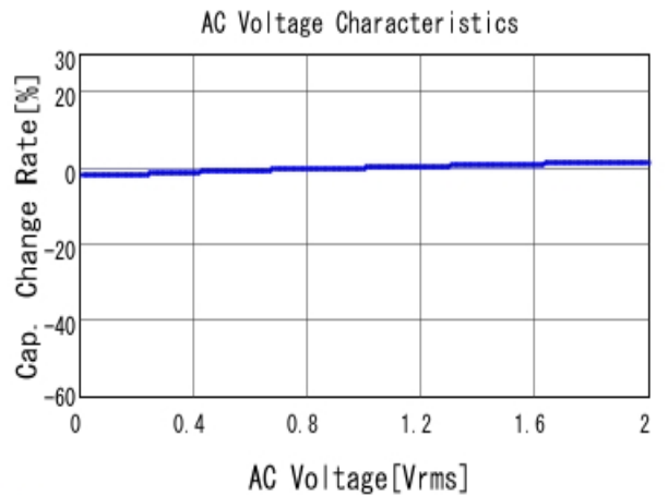
■ GRM188R72A222KA01 C-AC Voltage capchange, DCOV, 25.0d
