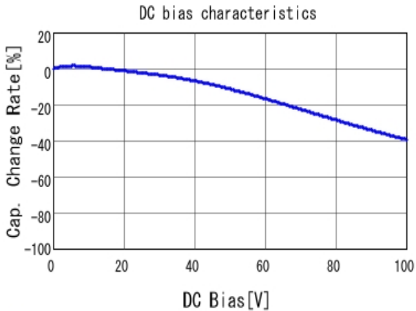
■ GRM188R72A152KA01 C-DC bias capchange, 25.0degC, AC1.
