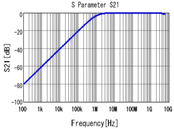
■ GRM188R72A152KA01 S21 DCOV, 25degC
