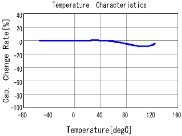
■ GRM188R72A152KA01 C-Temp. capchange, DCO. 0V, AC1.0Vrm
