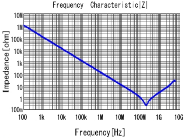
■ GRM188R72A152KA01 |Z| DCOV, 25degC
