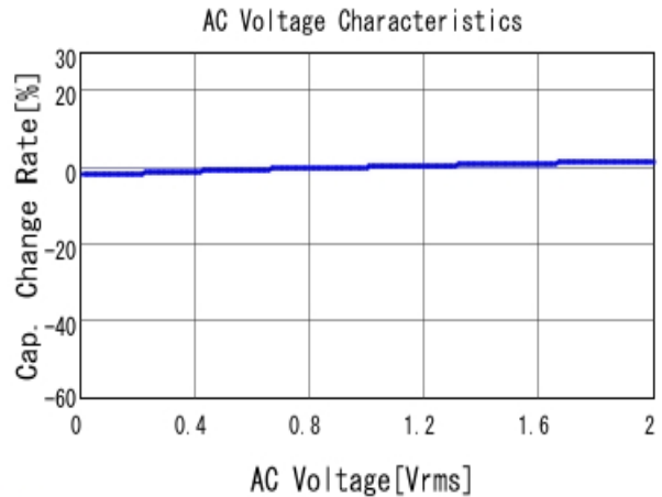
■ GRM188R72A152KA01 C-AC Voltage capchange, DCOV, 25.0d
