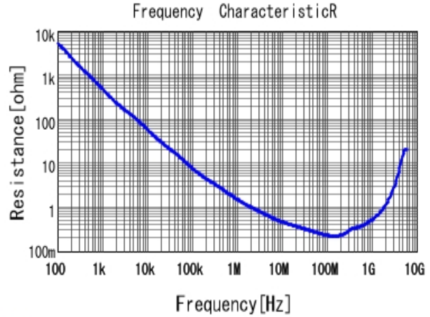
■ GRM188R72A152KA01 R DCOV, 25degC
