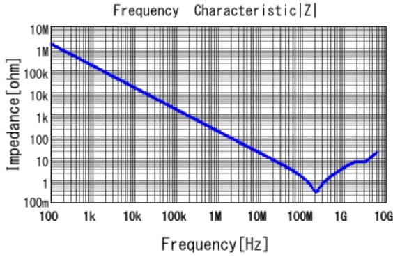
■ GRM188R72A102KA01 |Z| DCOV, 25degC
