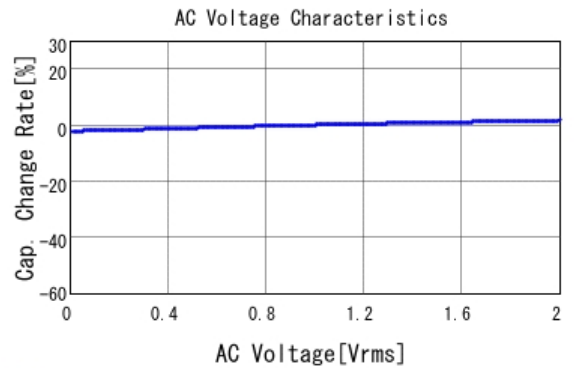
■ GRM188R72A102KA01 C-AC Voltage capchange, DCOV, 25.0d
