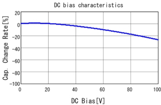
■ GRM188R72A102KA01 C-DC bias capchange, 25.0degC, AC1.
