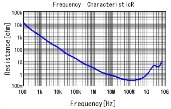
■ GRM188R72A102KA01 R DCOV, 25degC
