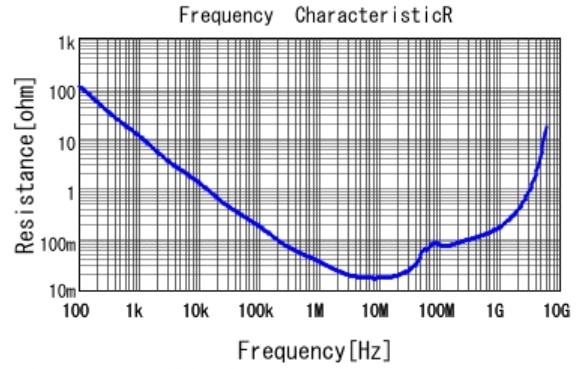
■ GRM188R71H683KA93 R DCOV, 25degC
