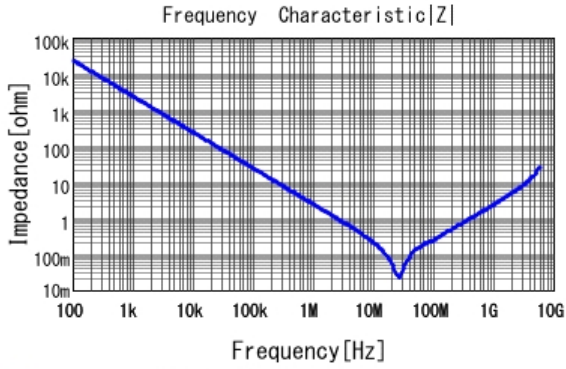
■ GRM188R71H683KA93 |Z| DCOV, 25degC
