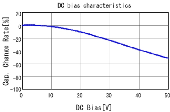
■ GRM188R71H683KA93 C-DC bias capchange, 25.0degC, AC1.
