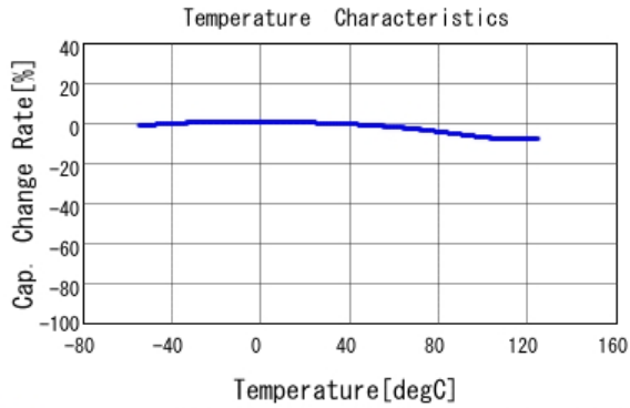
■ GRM188R71H683KA93 C-Temp. capchange, DC0.0V, AC1.0V rm
