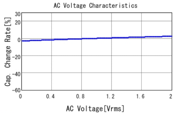
■ GRM188R71H683KA93 C-AC Voltage capchange, DCOV, 25.0d
