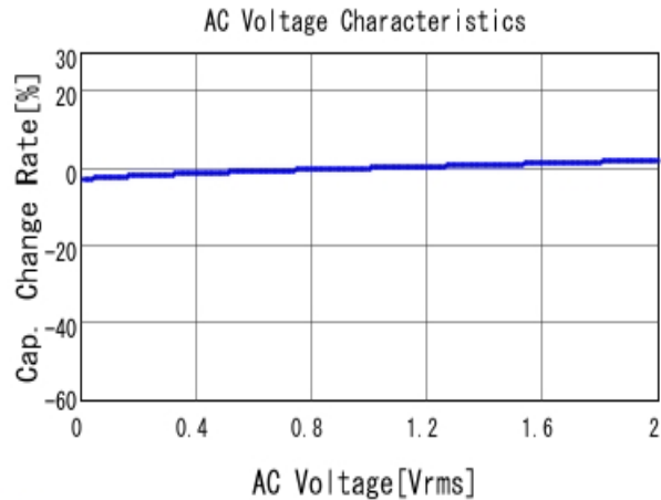
■ GRM188R71H682KA01 C-AC Voltage capchange, DCOV, 25.0d
