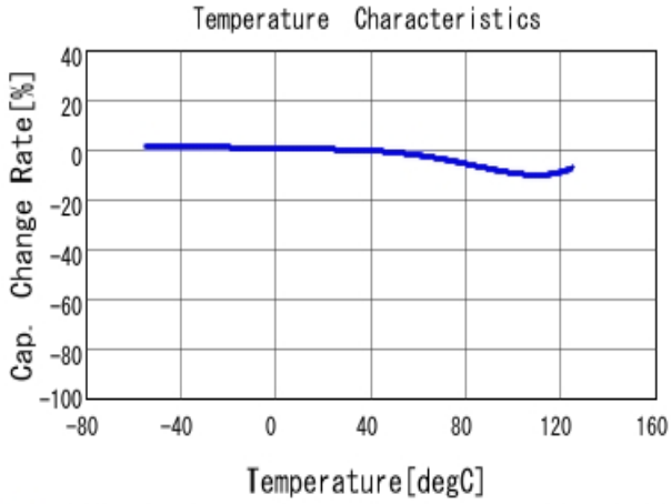
■ GRM188R71H682KA01 C-Temp. capchange, DCO. 0V, AC1.0V rm
