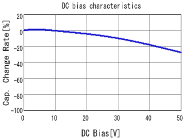
■ GRM188R71H682KA01 C-DC bias capchange, 25.0degC, AC1.
