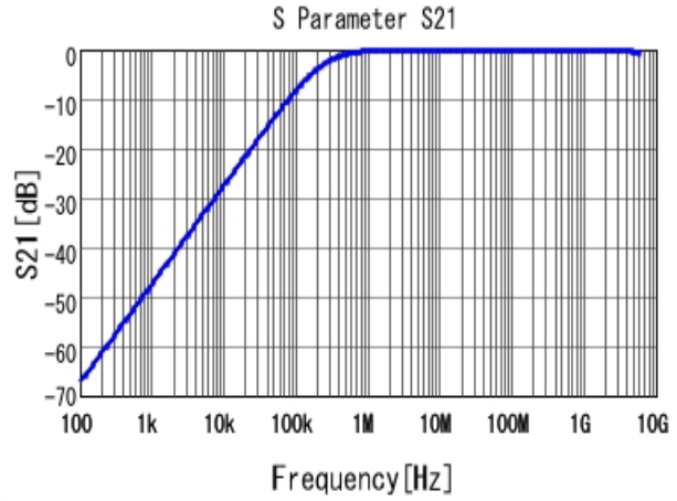
■ GRM188R71H682KA01 S21 DCOV, 25degC
