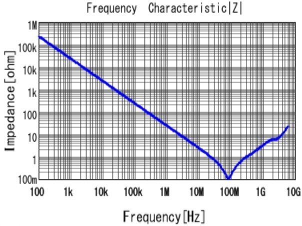
■ GRM188R71H682KA01 |Z| DCOV, 25degC
