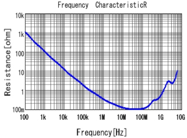
■ GRM188R71H682KA01 R DCOV, 25degC
