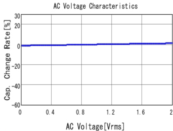
■ GRM188R71H681KA01 C-AC Voltage capchange, DCOV, 25.0d
