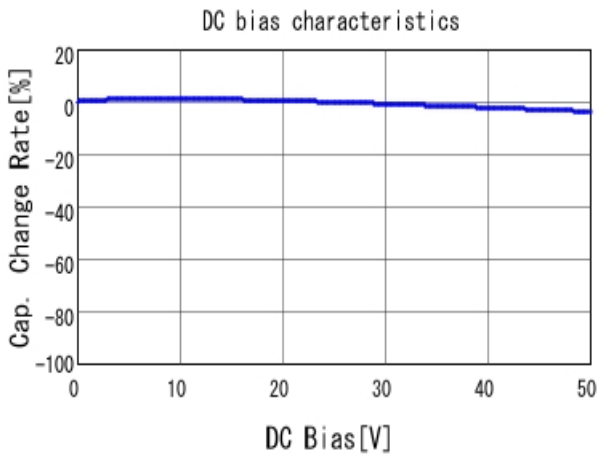
■ GRM188R71H681KA01 C-DC bias capchange, 25.0degC, AC1.
