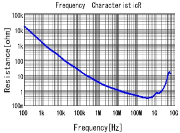
■ GRM188R71H681KA01 R DCOV, 25degC
