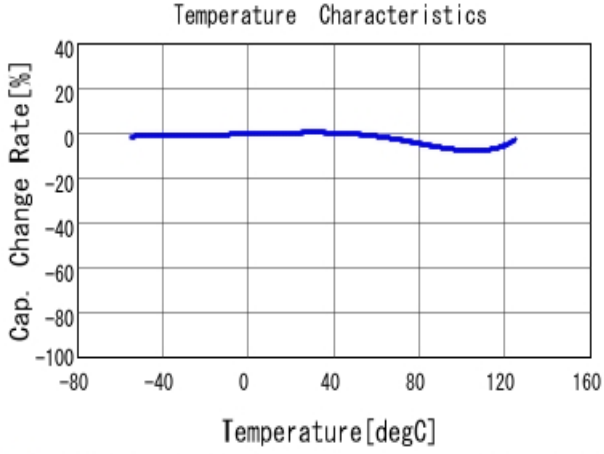
■ GRM188R71H681KA01 C-Temp. capchange, DCO. 0V, AC1.0Vrm
