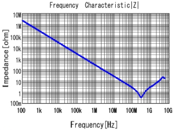
■ GRM188R71H681KA01 |Z| DCOV, 25degC
