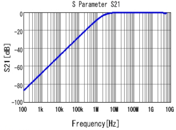
■ GRM188R71H681KA01 S21 DCOV, 25degC
