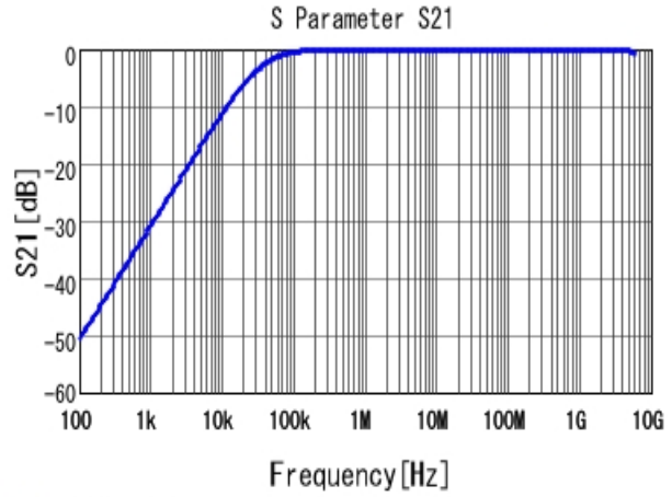
■ GRM188R71H473KA61 S21 DCOV, 25degC
