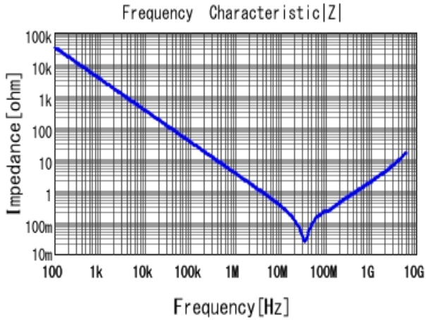
■ GRM188R71H473KA61 |Z| DCOV, 25degC
