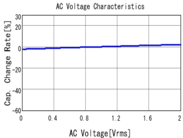
■ GRM188R71H473KA61 C-AC Voltage capchange, DCOV, 25.0d
