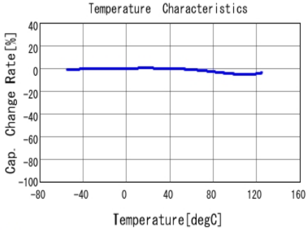
■ GRM188R71H473KA61 C-Temp. capchange, DCO. 0V, AC1.0V rm
