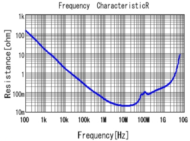
■ GRM188R71H473KA61 R DCOV, 25degC
