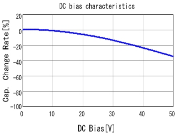
■ GRM188R71H473KA61 C-DC bias capchange, 25.0degC, AC1.
