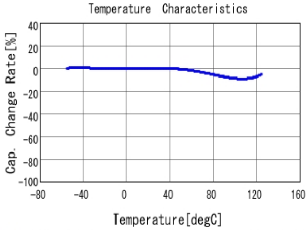
■ GRM188R71H472KA01 C-Temp. capchange, DCO. 0V, AC1.0Vrm
