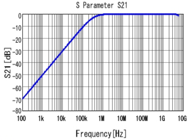
■ GRM188R71H472KA01 S21 DCOV, 25degC
