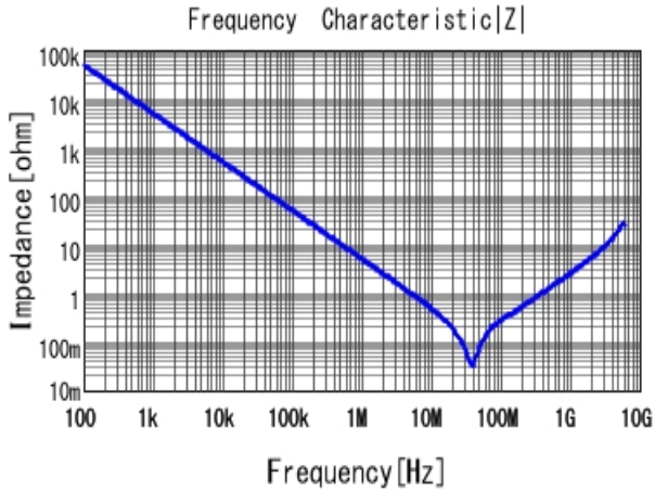
■ GRM188R71H333KA61 |Z| DCOV, 25degC
