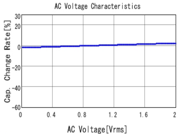
■ GRM188R71H333KA61 C-AC Voltage capchange, DCOV, 25.0d
