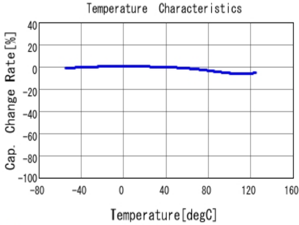
■ GRM188R71H333KA61 C-Temp. capchange, DCO. 0V, AC1.0V rm
