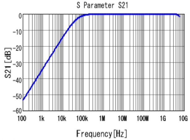
■ GRM188R71H333KA61 S21 DCOV, 25degC
