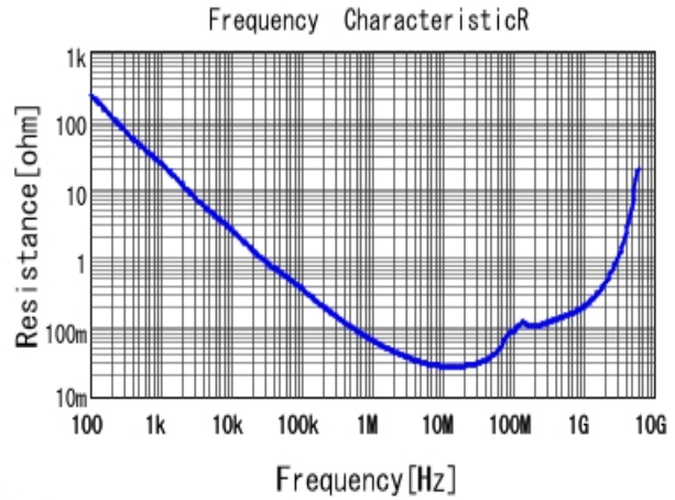
■ GRM188R71H333KA61 R DCOV, 25degC
