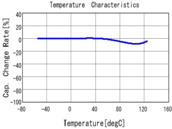
■ GRM188R71H332KA01 C-Temp. capchange, DCO. 0V, AC1.0Vrm
