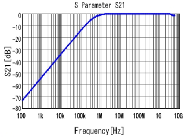
■ GRM188R71H332KA01 S21 DCOV, 25degC
