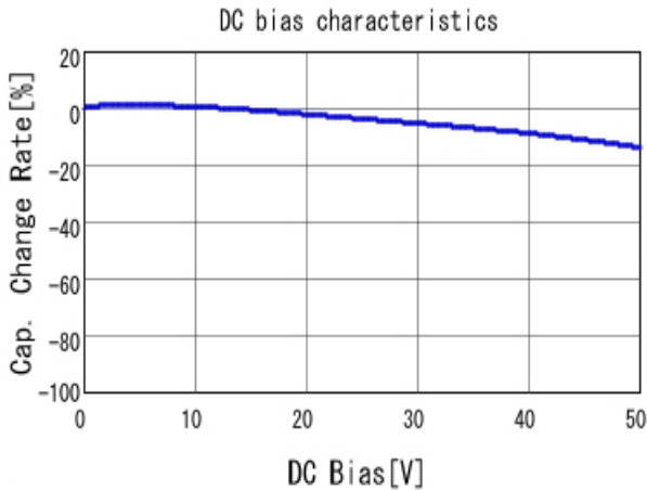
■ GRM188R71H332KA01 C-DC bias capchange, 25.0degC, AC1.
