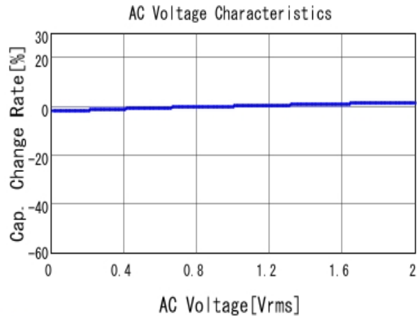
■ GRM188R71H332KA01 C-AC Voltage capchange, DCOV, 25.0d
