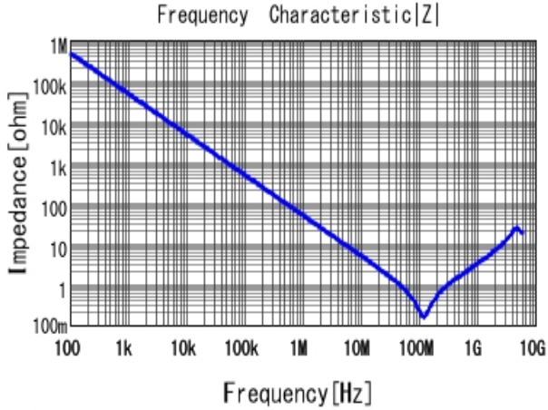
■ GRM188R71H332KA01 |Z| DCOV, 25degC
