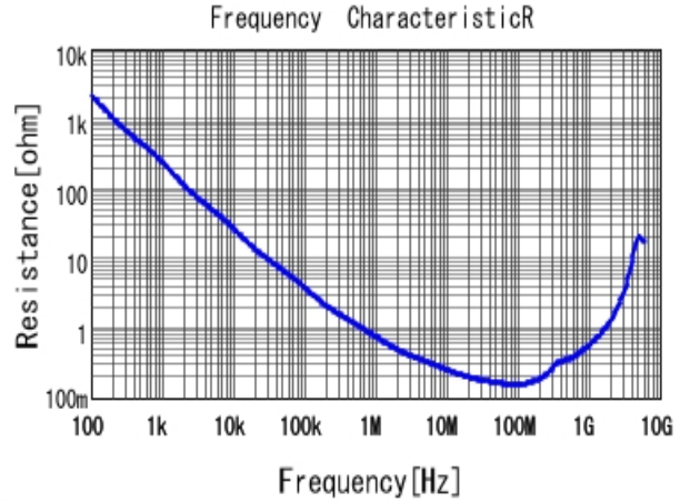
■ GRM188R71H332KA01 R DCOV, 25degC
