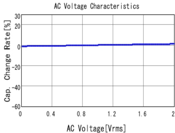
■ GRM188R71H331KA01 C-AC Voltage capchange, DCOV, 25.0d
