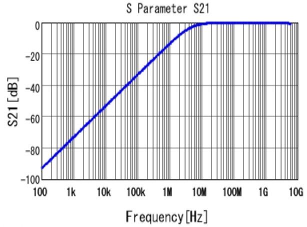
■ GRM188R71H331KA01 S21 DCOV, 25degC
