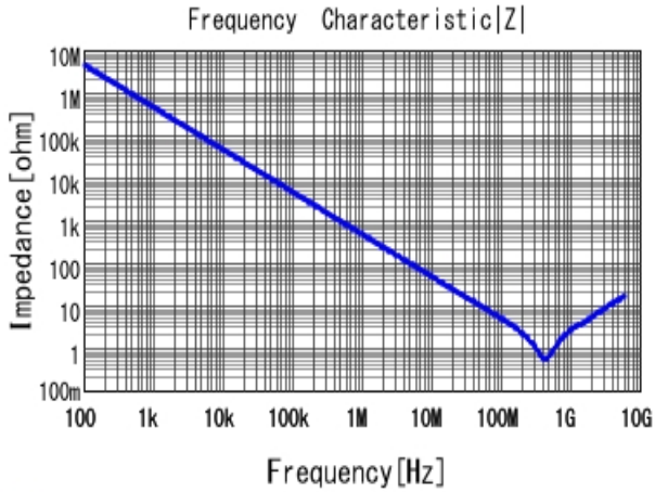
■ GRM188R71H331KA01 |Z| DCOV, 25degC
