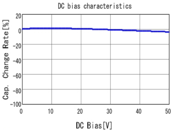
■ GRM188R71H331KA01 C-DC bias capchange, 25.0degC, AC1.
