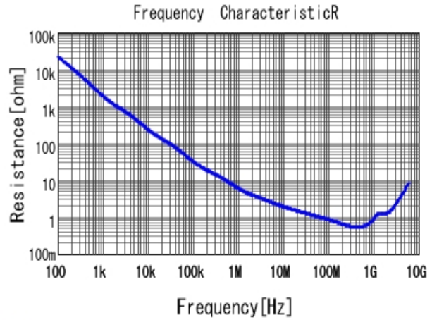
■ GRM188R71H331KA01 R DCOV, 25degC
