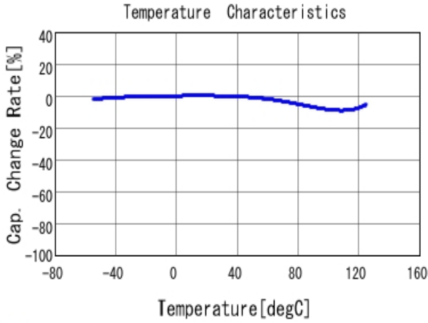
■ GRM188R71H331KA01 C-Temp. capchange, DCO. 0V, AC1.0V rm
