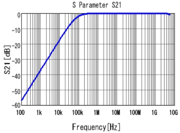
■ GRM188R71H223KA01 S21 DCOV, 25degC
