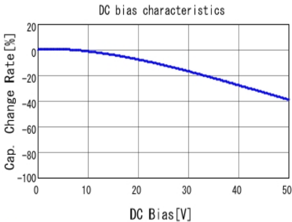
■ GRM188R71H223KA01 C-DC bias capchange, 25.0degC, AC1.
