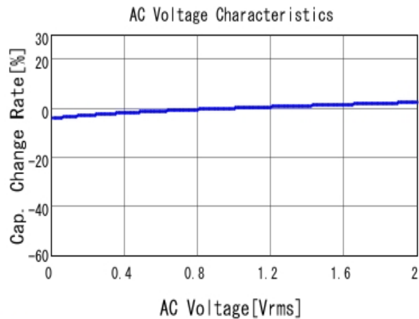
■ GRM188R71H223KA01 C-AC Voltage capchange, DCOV, 25.0d
