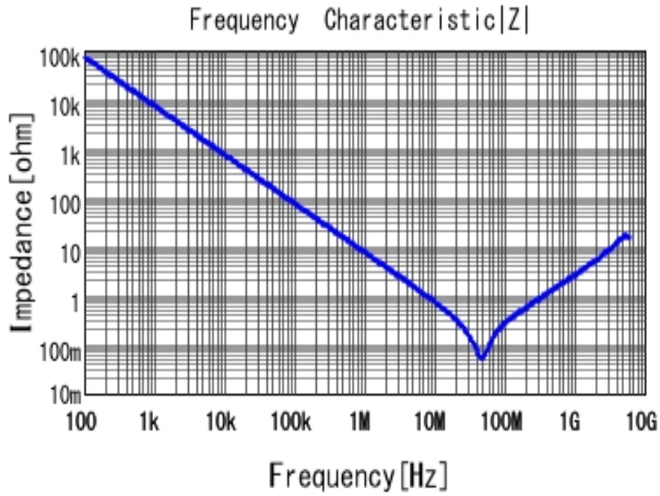
■ GRM188R71H223KA01 |Z| DCOV, 25degC
