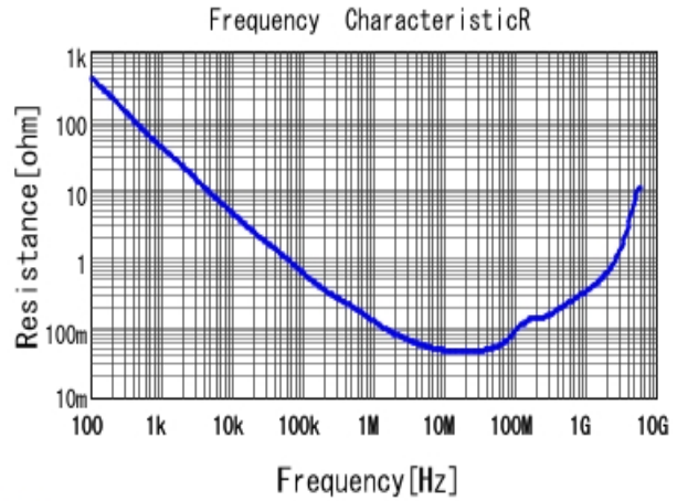
■ GRM188R71H223KA01 R DCOV, 25degC
