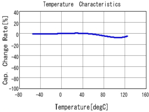
■ GRM188R71H223KA01 C-Temp. capchange, DCO. 0V, AC1.0Vrm
