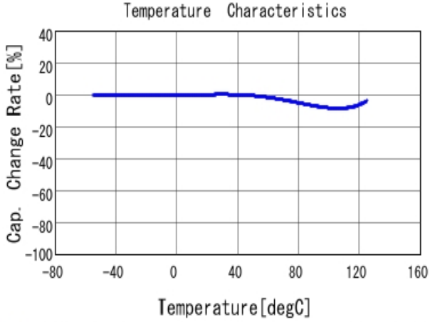
■ GRM188R71H222KA01 C-Temp. capchange, DCO. 0V, AC1.0Vrm
