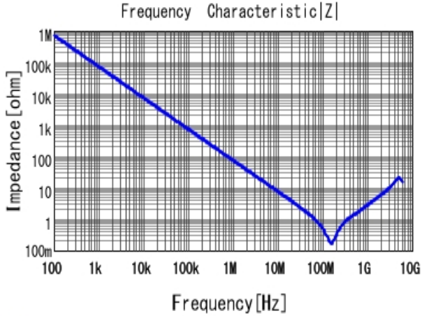
■ GRM188R71H222KA01 |Z| DCOV, 25degC
