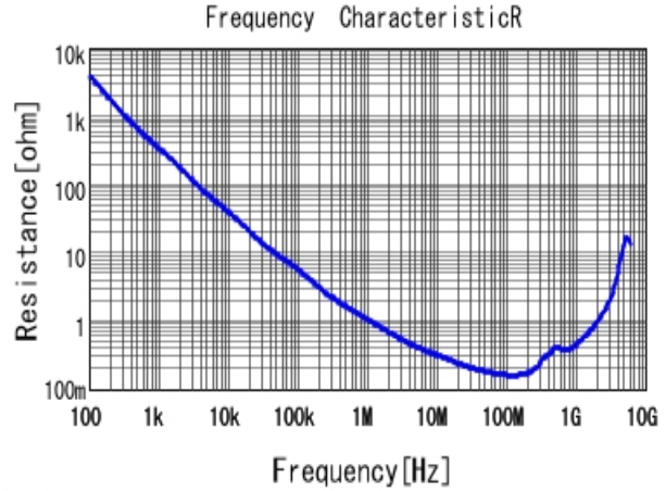
■ GRM188R71H222KA01 R DCOV, 25degC
