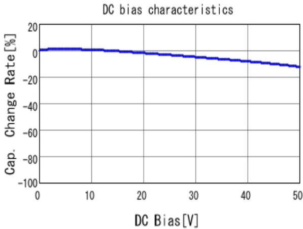
■ GRM188R71H222KA01 C-DC bias capchange, 25.0degC, AC1.
