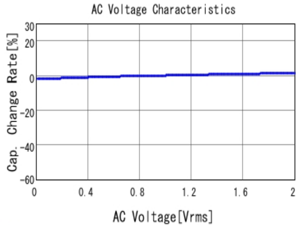
■ GRM188R71H222KA01 C-AC Voltage capchange, DCOV, 25.0d
