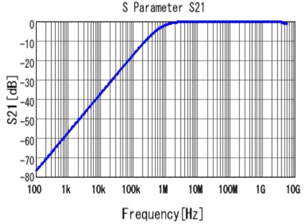
■ GRM188R71H222KA01 S21 DCOV, 25degC
