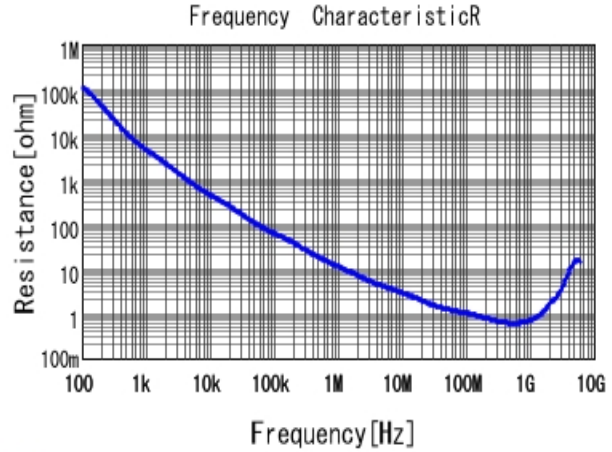
■ GRM188R71H221KA01 R DCOV, 25degC
