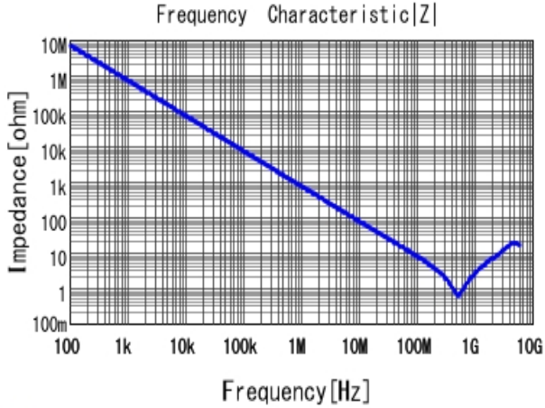
■ GRM188R71H221KA01 |Z| DCOV, 25degC
