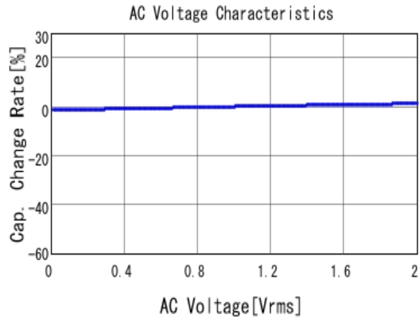
■ GRM188R71H221KA01 C-AC Voltage capchange, DCOV, 25.0d
