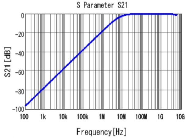
■ GRM188R71H221KA01 S21 DCOV, 25degC
