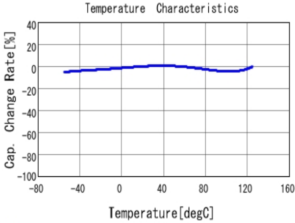
■ GRM188R71H221KA01 C-Temp. capchange, DCO. 0V, AC1.0V rm
