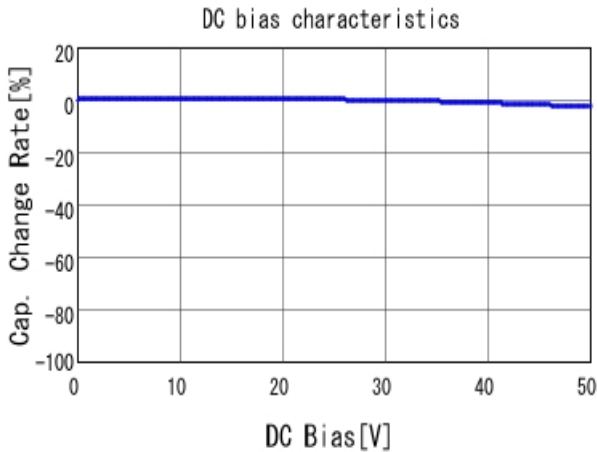
■ GRM188R71H221KA01 C-DC bias capchange, 25.0degC, AC1.
