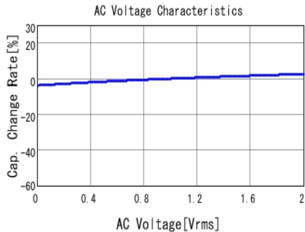
■ GRM188R71H154KAC4 C-AC Voltage capchange, DCOV, 25.0d
