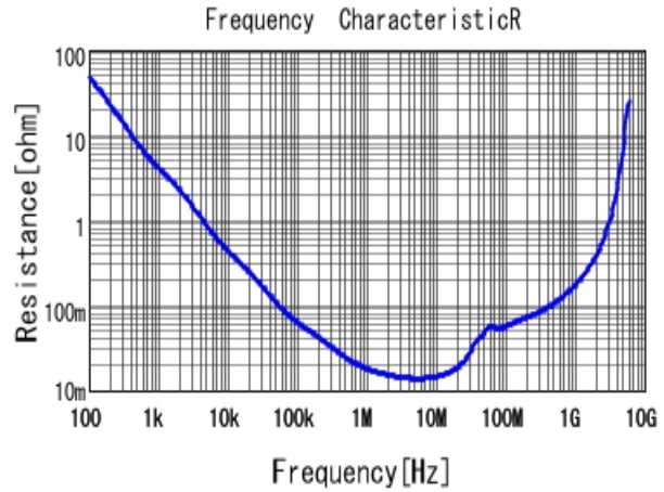
■ GRM188R71H154KAC4 R DCOV, 25degC
