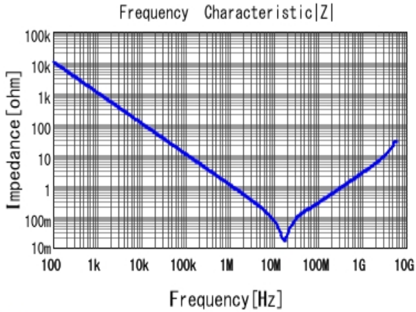
■ GRM188R71H154KAC4 |Z| DCOV, 25degC
