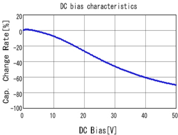
■ GRM188R71H154KAC4 C-DC bias capchange, 25.0degC, AC1.
