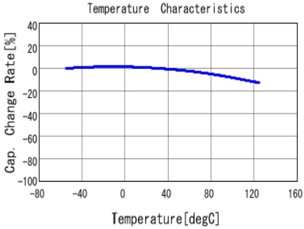
■ GRM188R71H154KAC4 C-Temp. capchange, DCO. 0V, AC1.0V rm
