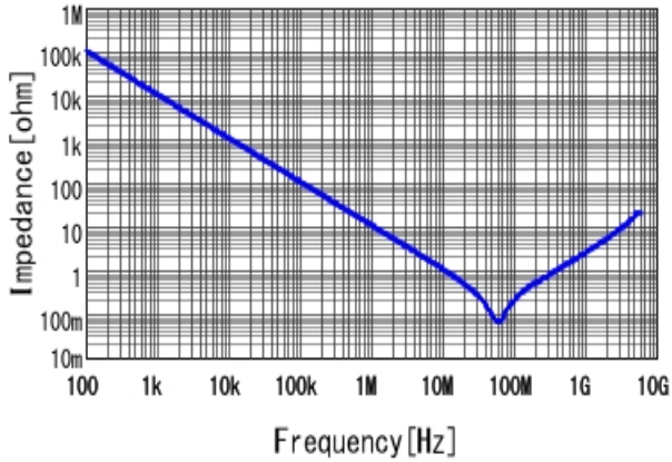
■ GRM188R71H153KA01 |Z| DCOV, 25degC
