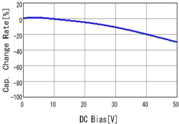
■ GRM188R71H153KA01 C-DC bias capchange, 25.0degC, AC1.
