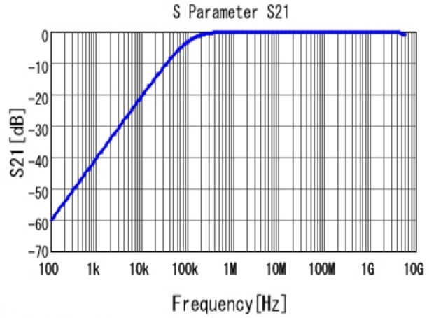
■ GRM188R71H153KA01 S21 DCOV, 25degC
