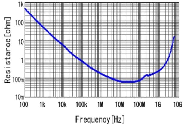
■ GRM188R71H153KA01 R DCOV, 25degC
