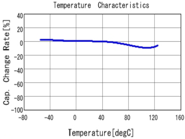
■ GRM188R71H153KA01 C-Temp. capchange, DCO. 0V, AC1.0Vrm
