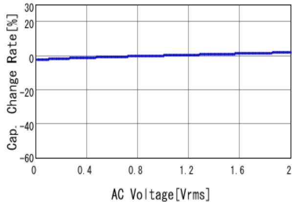
■ GRM188R71H153KA01 C-AC Voltage capchange, DCOV, 25.0d
