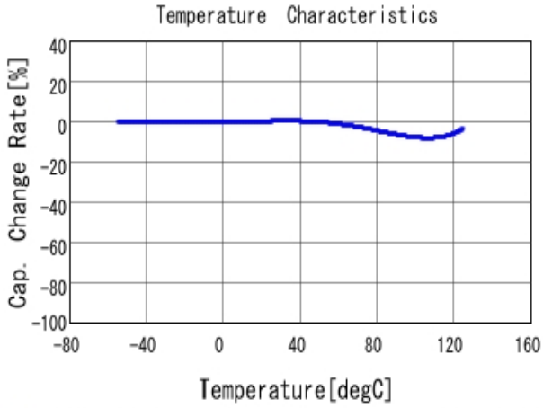
■ GRM188R71H152KA01 C-Temp. capchange, DCO. 0V, AC1.0Vrm
