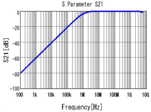
■ GRM188R71H152KA01 S21 DCOV, 25degC
