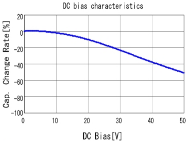
■ GRM188R71H104KA93 C-DC bias capchange, 25.0degC, AC1.
