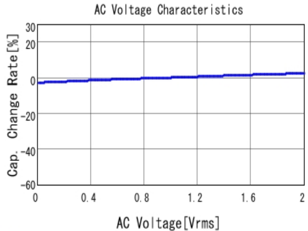
■ GRM188R71H104KA93 C-AC Voltage capchange, DCOV, 25.0d
