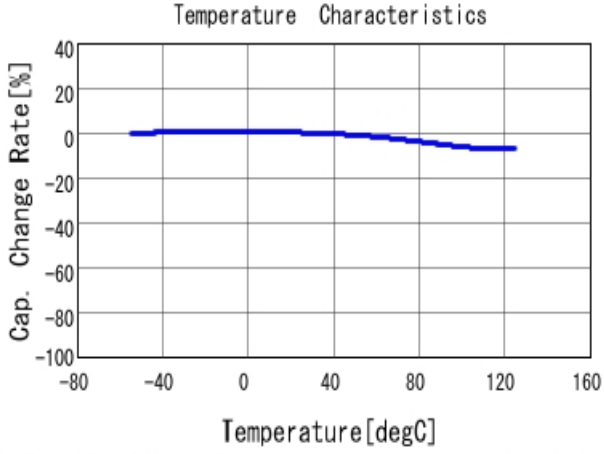
■ GRM188R71H104KA93 C-Temp. capchange, DC0.0V, AC1.0V r m
