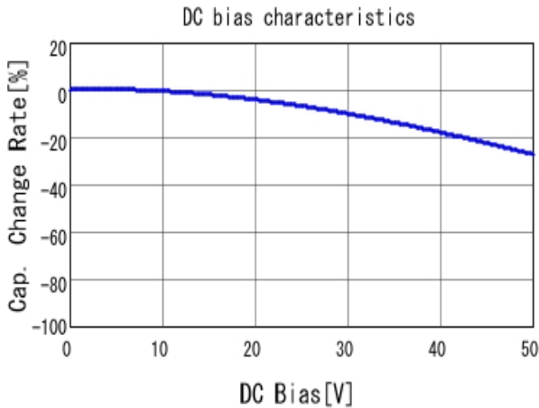
■ GRM188R71H103KA01 C-DC bias capchange, 25.0degC, AC1.
