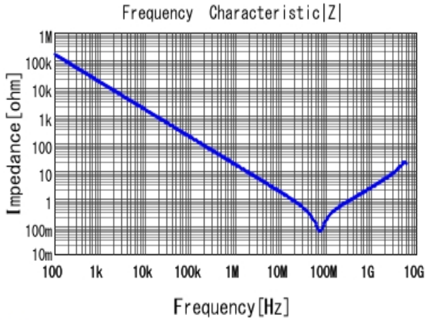
■ GRM188R71H103KA01 |Z| DCOV, 25degC
