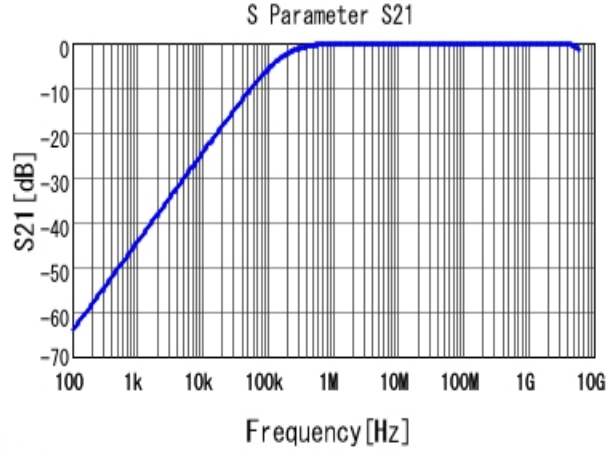
■ GRM188R71H103KA01 S21 DCOV, 25degC
