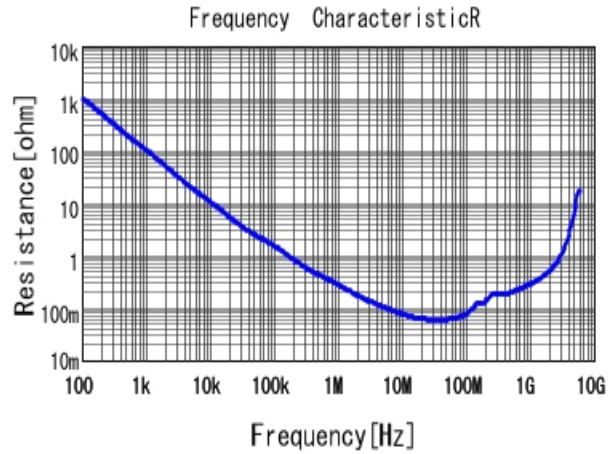
■ GRM188R71H103KA01 R DCOV, 25degC
