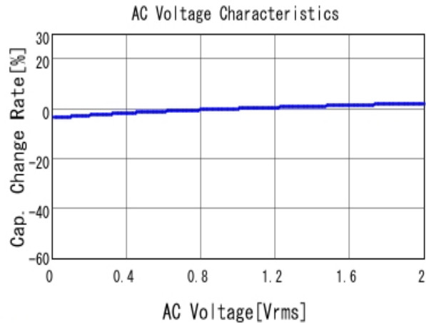
■ GRM188R71H103KA01 C-AC Voltage capchange, DCOV, 25.0d
