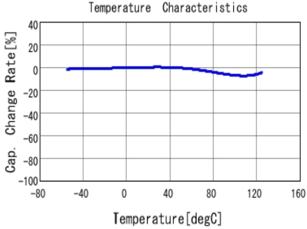
■ GRM188R71H103KA01 C-Temp. capchange, DCO. 0V, AC1.0Vrm
