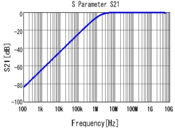
■ GRM188R71H102KA01 S21 DCOV, 25degC
