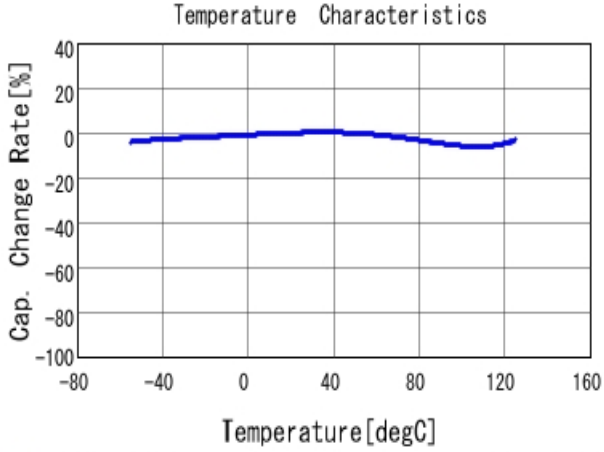
■ GRM188R71H102KA01 C-Temp. capchange, DCO. 0V, AC1.0Vrm
