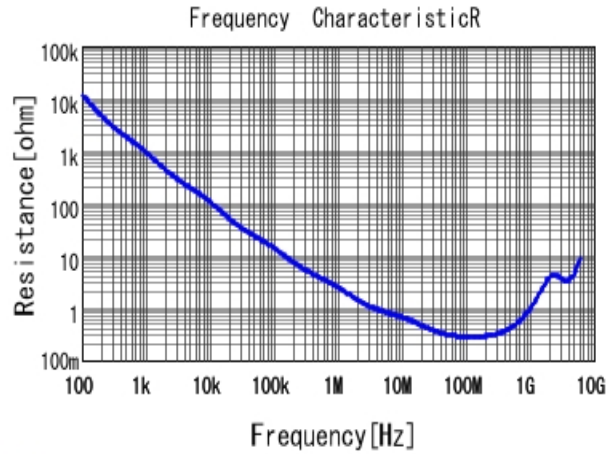
■ GRM188R71H102KA01 R DCOV, 25degC
