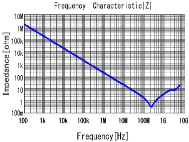
■ GRM188R71H102KA01 |Z| DCOV, 25degC
