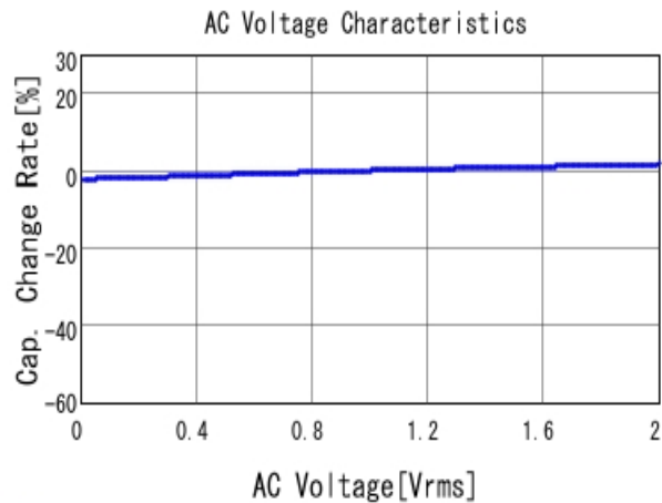
■ GRM188R71H102KA01 C-AC Voltage capchange, DCOV, 25.0d
