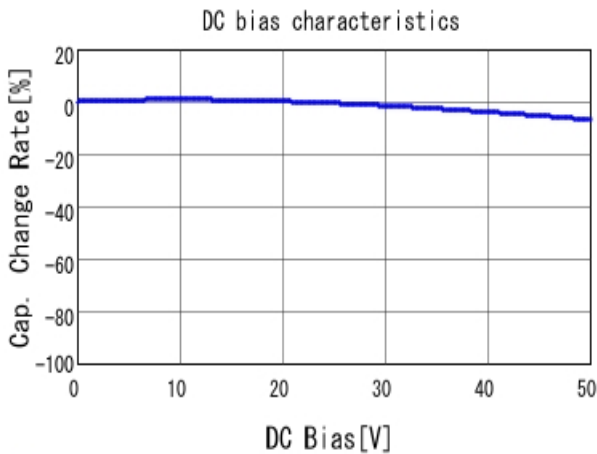
■ GRM188R71H102KA01 C-DC bias capchange, 25.0degC, AC1.
