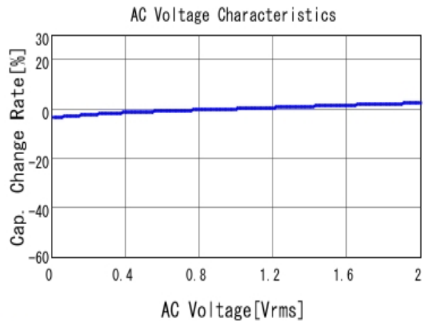
■ GRM188R71E473KA01 C-AC Voltage capchange, DCOV, 25.0d
