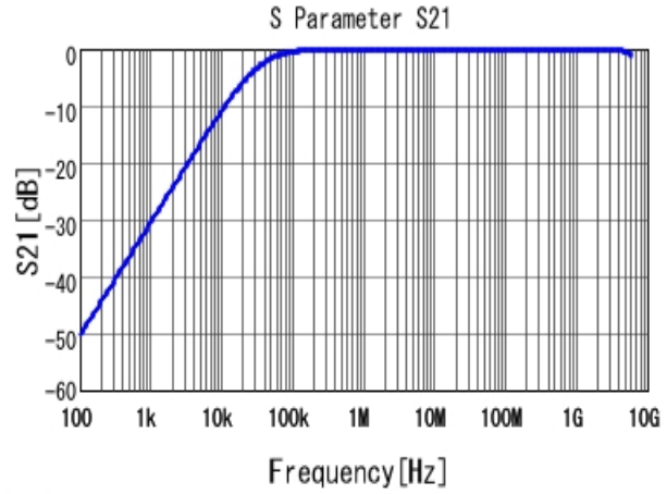
■ GRM188R71E473KA01 S21 DCOV, 25degC
