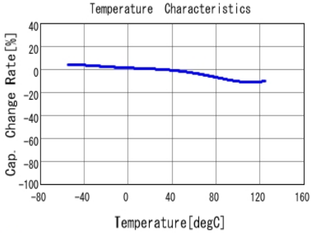
■ GRM188R71E473KA01 C-Temp. capchange, DCO. 0V, AC1.0V rm
