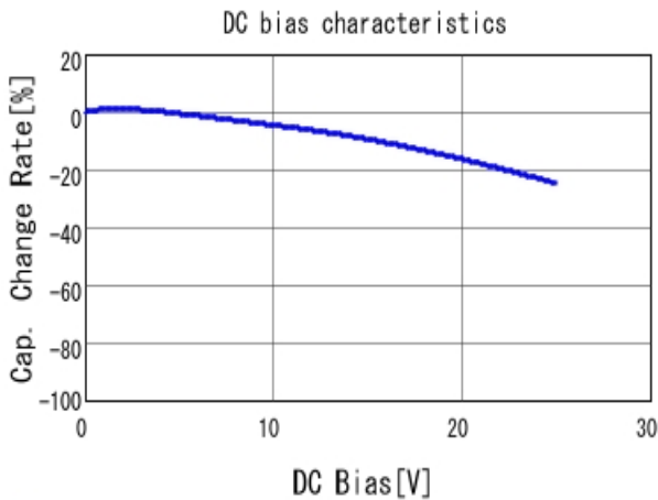
■ GRM188R71E473KA01 C-DC bias capchange, 25.0degC, AC1.
