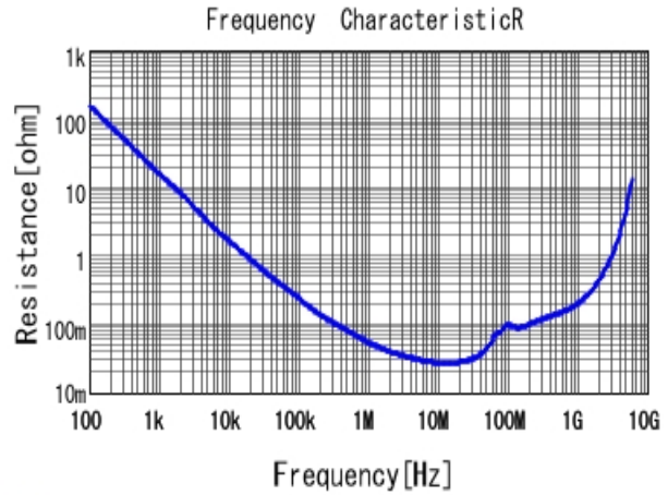
■ GRM188R71E473KA01 R DCOV, 25degC
