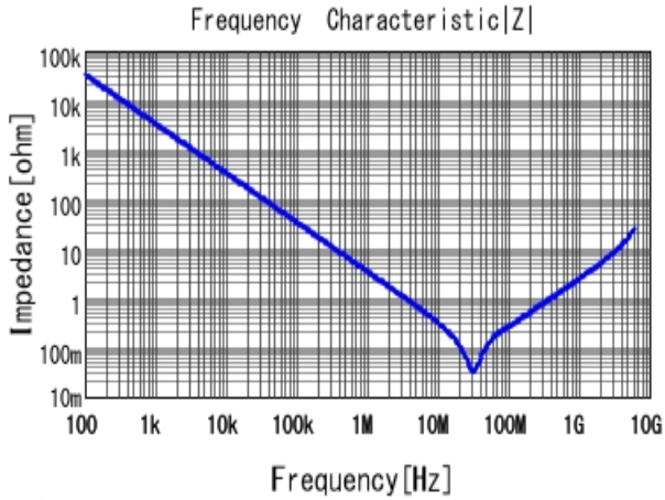
■ GRM188R71E473KA01 |Z| DCOV, 25degC
