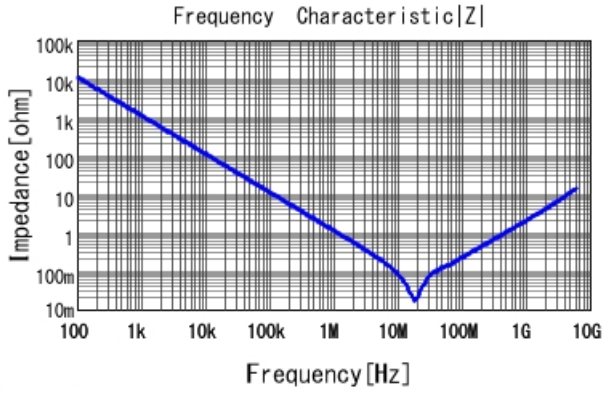
GRM188R71E154KA01 |Z| DCOV, 25degC
