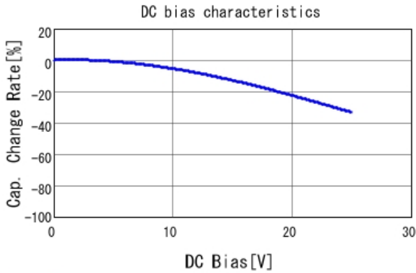
GRM188R71E154KA01 C-DC bias capchange, 25.0degC, A
