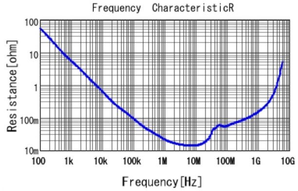
GRM188R71E154KA01 R DCOV, 25degC
