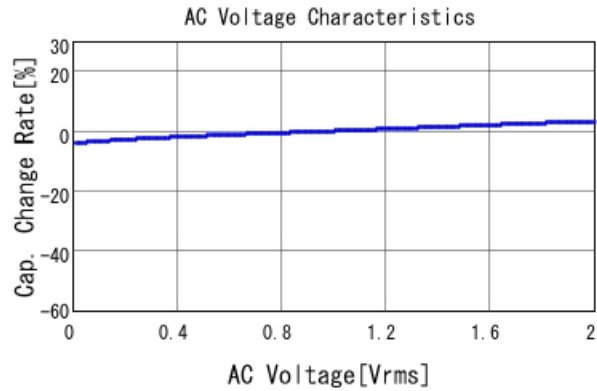
GRM188R71E154KA01 C-AC Voltage capchange, DCOV, 25
