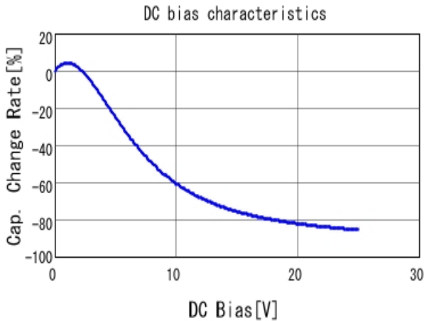
■ GRM188R71E105KA12 C-DC bias capchange, 25.0degC, AC1.
