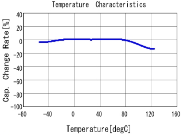
■ GRM188R71E105KA12 C-Temp. capchange, DC0.0V, AC1.0V rm
