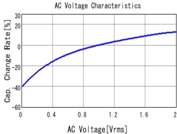
■ GRM188R71E105KA12 C-AC Voltage capchange, DCOV, 25.0d
