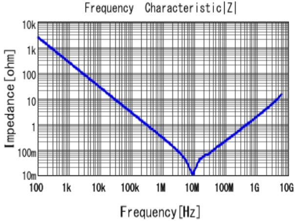
■ GRM188R71E105KA12 |Z| DCOV, 25degC
