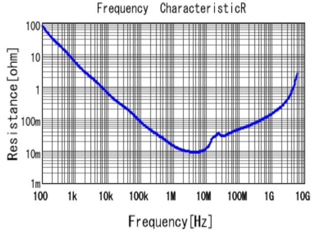
■ GRM188R71E105KA12 R DCOV, 25degC
