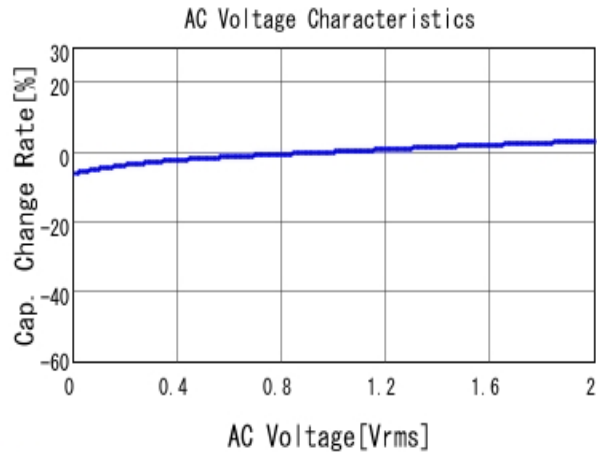
■ GRM188R71E104KA01 C-AC Voltage capchange, DCOV, 25.0d
