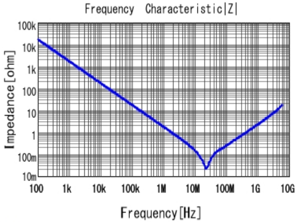
■ GRM188R71E104KA01 |Z| DCOV, 25degC
