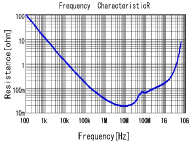
■ GRM188R71E104KA01 R DCOV, 25degC
