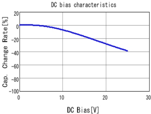
■ GRM188R71E104KA01 C-DC bias capchange, 25.0degC, AC1.
