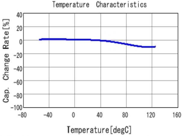
■ GRM188R71E104KA01 C-Temp. capchange, DC0.0V, AC1.0V rm
