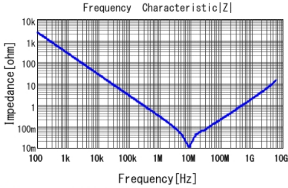
■ GRM188R71C105KA12 |Z| DCOV, 25degC
