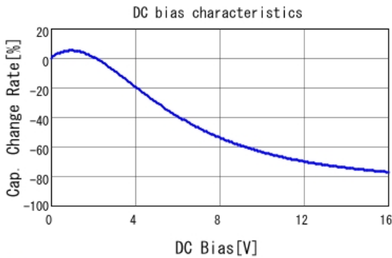
■ GRM188R71C105KA12 C-DC bias capchange, 25.0degC, AC1.
