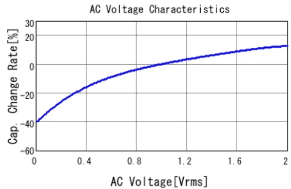
■ GRM188R71C105KA12 C-AC Voltage capchange, DCOV, 25.0d
