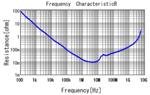
■ GRM188R71C105KA12 R DCOV, 25degC
