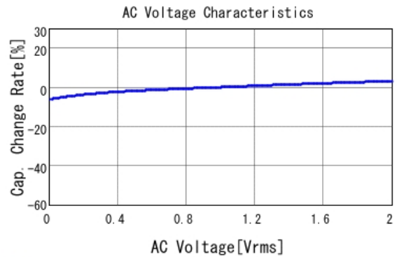
■ GRM188R71C104KA01 C-AC Voltage capchange, DCOV, 25.0d
