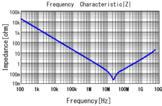
■ GRM188R71C104KA01 |Z| DCOV, 25degC
