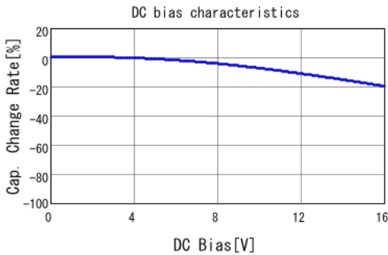
■ GRM188R71C104KA01 C-DC bias capchange, 25.0degC, AC1.
