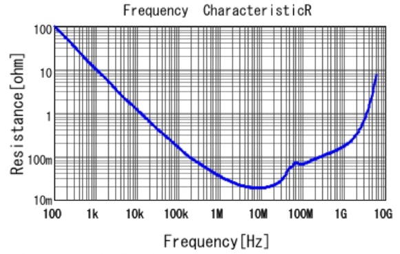
■ GRM188R71C104KA01 R DCOV, 25degC
