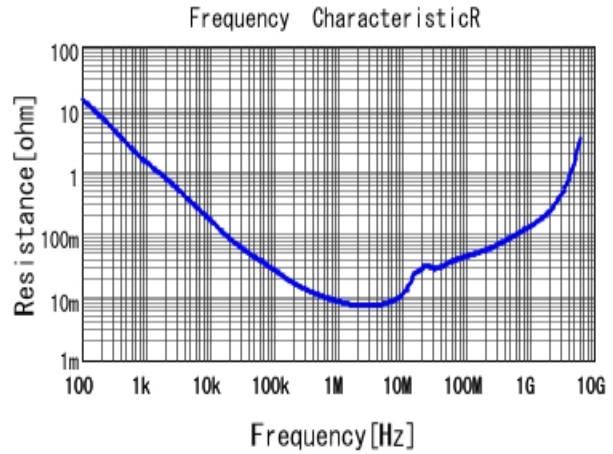
■ GRM188R71A684KA61 R DCOV, 25degC
