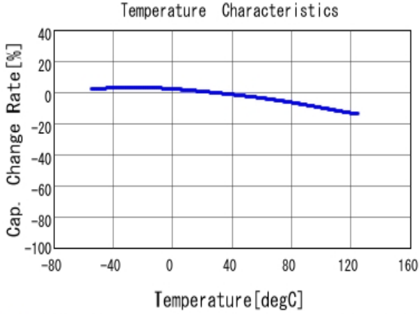
■ GRM188R71A684KA61 C-Temp. capchange, DC0.0V, AC1.0V r m
