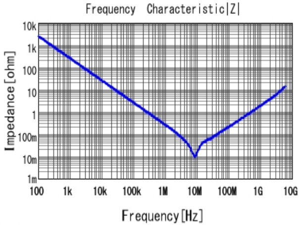
■ GRM188R71A684KA61 |Z| DCOV, 25degC
