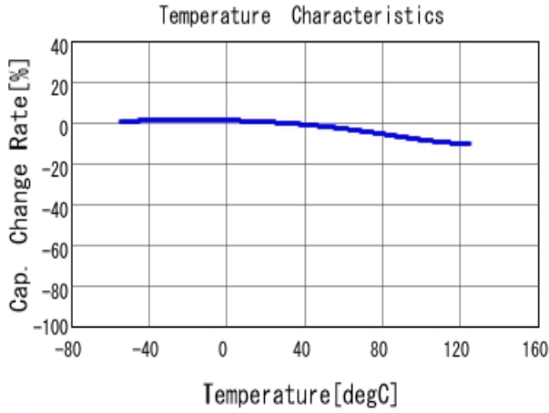
■ GRM188R71A334KA61 C-Temp. capchange, DC0.0V, AC1.0V r m
