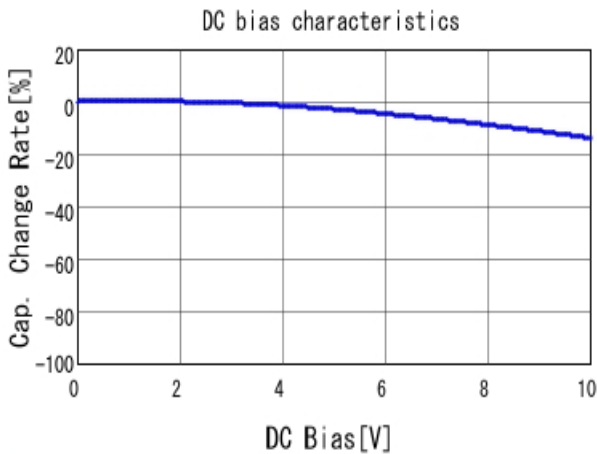
■ GRM188R71A334KA61 C-DC bias capchange, 25.0degC, AC1.
