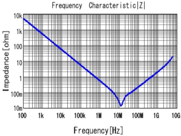
■ GRM188R71A334KA61 |Z| DCOV, 25degC
