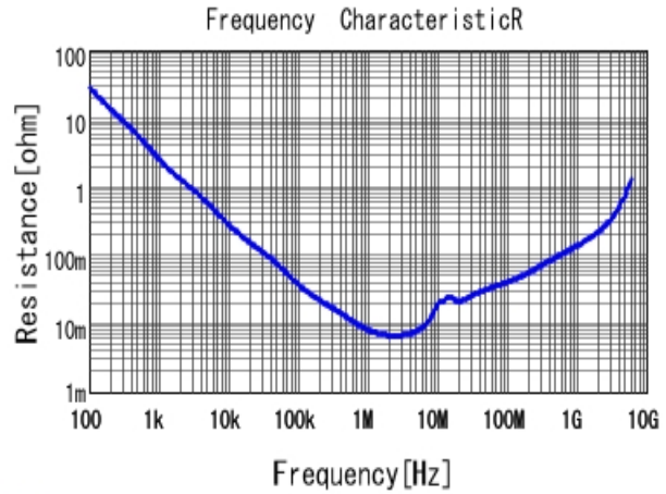
■ GRM188R71A225KE15 R DCOV, 25degC
