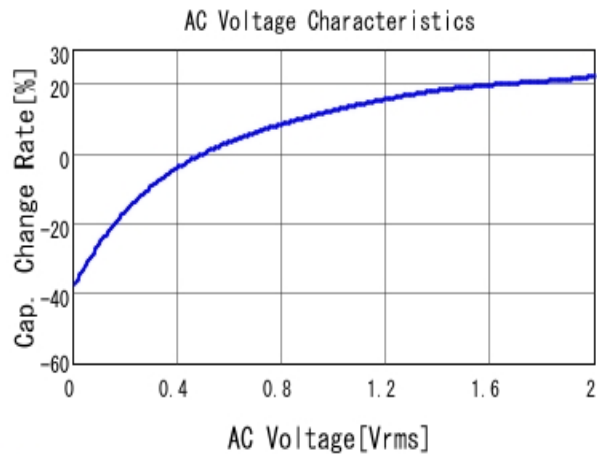
■ GRM188R71A225KE15 C-AC Voltage capchange, DCOV, 25.0d
