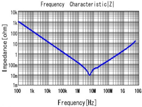
■ GRM188R71A225KE15 |Z| DCOV, 25degC
