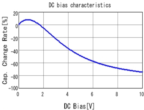
■ GRM188R71A225KE15 C-DC bias capchange, 25.0degC, AC0.
