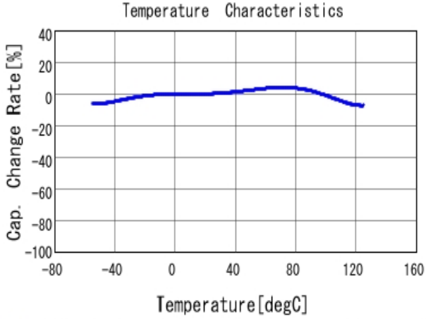
■ GRM188R71A225KE15 C-Temp. capchange, DCO. 0V, ACO. 5V rm
