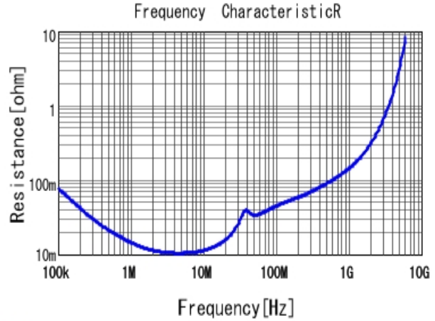
■ GRM188R71A224KA01 R DCOV, 25degC
