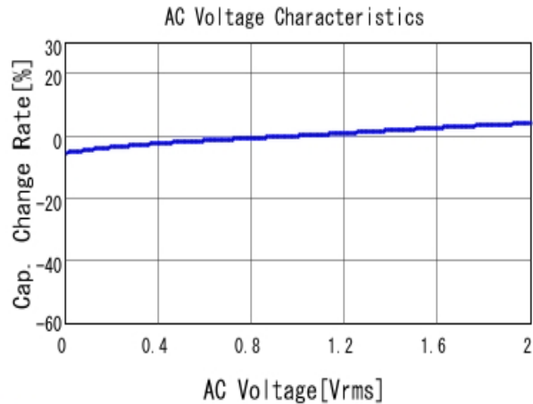
■ GRM188R71A224KA01 C-AC Voltage capchange, DCOV, 25.0d
