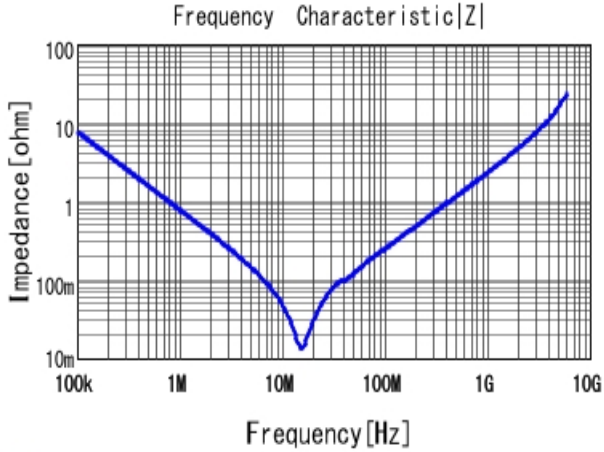
■ GRM188R71A224KA01 |Z| DCOV, 25degC
