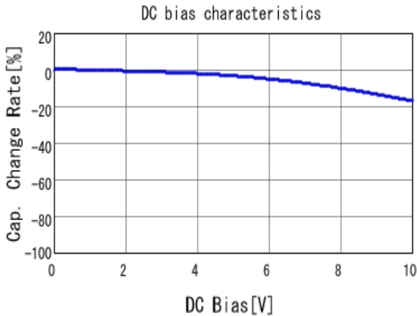
■ GRM188R71A224KA01 C-DC bias capchange, 25.0degC, AC1.
