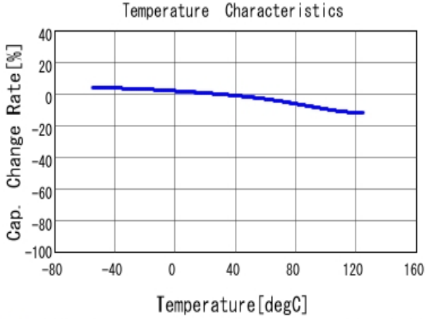
■ GRM188R71A224KA01 C-Temp. capchange, DC0.0V, AC1.0V rm
