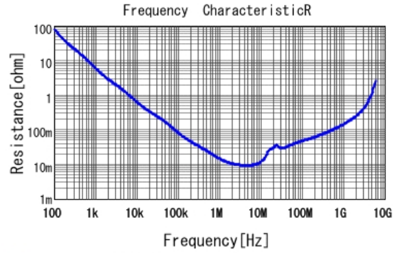
■ GRM188R71A105KA61 R DCOV, 25degC
