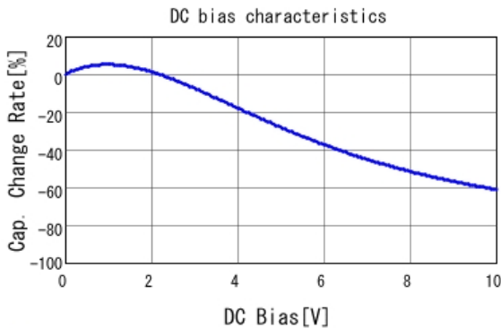
■ GRM188R71A105KA61 C-DC bias capchange, 25.0degC, AC1.
