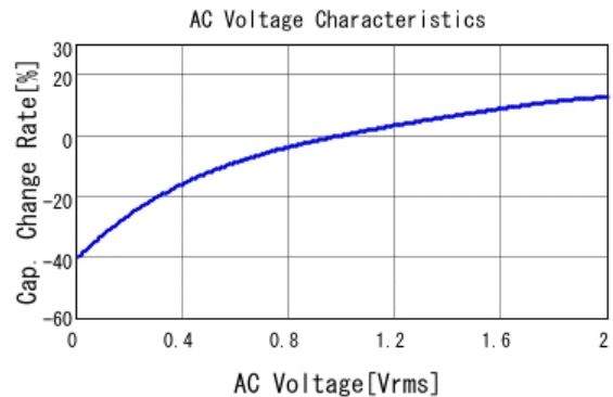
■ GRM188R71A105KA61 C-AC Voltage capchange, DCOV, 25.0d
