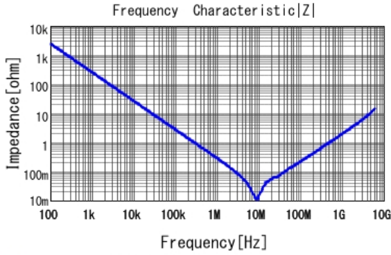
■ GRM188R71A105KA61 |Z| DCOV, 25degC
