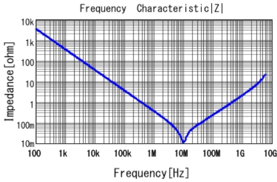
■ GRM188R70J474KA01 |Z| DCOV, 25degC
