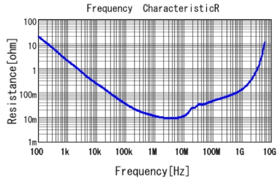
■ GRM188R70J474KA01 R DCOV, 25degC
