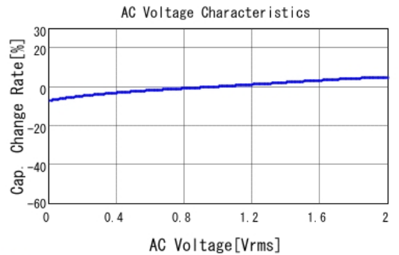
■ GRM188R70J474KA01 C-AC Voltage capchange, DCOV, 25.0d
