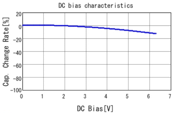
■ GRM188R70J474KA01 C-DC bias capchange, 25.0degC, AC1.
