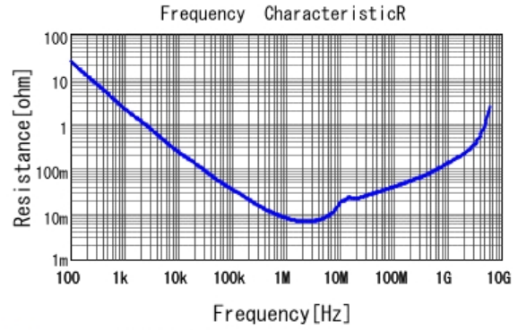
■ GRM188R6YA225KA12 R DCOV, 25degC
