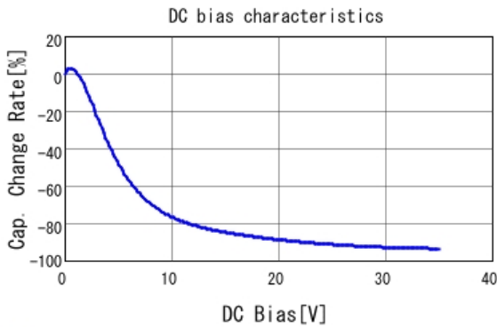
■ GRM188R6YA225KA12 C-DC bias capchange, 25.0degC, AC1.
