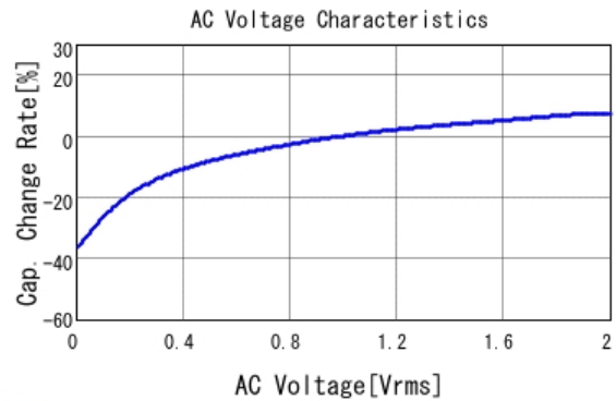
■ GRM188R6YA225KA12 C-AC Voltage capchange, DCOV, 25.0d
