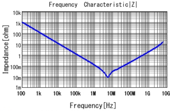
■ GRM188R6YA225KA12 |Z| DCOV, 25degC
